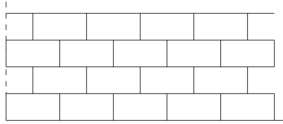
Fig. 1. The wall tiling of \mathbb{N}^2 .
