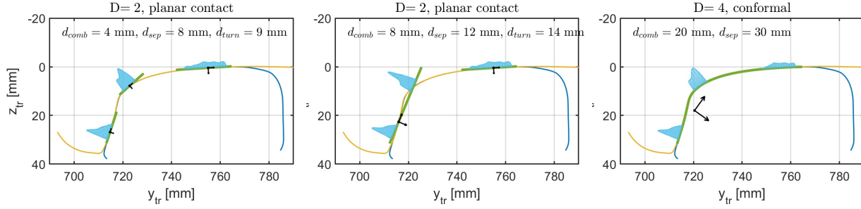
Figure 3.10: Illustration of ‘contact patches’ with local coordinate systems used for the solution. Multiple ‘interpenetration regions’ may be combined into a single ‘patch’ if the distance and angle difference are smaller than the threshold values.
