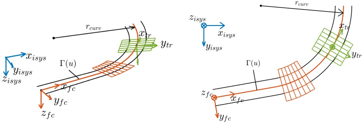
Figure 3.2: Left: perspective view, right: top view on the track, illustrating a track curve \Gamma(u) with ‘fixed curvilinear’ track coordinates ‘fc’ (red) versus ‘moving rectilinear’ track coordinates ‘tr’ (green).
