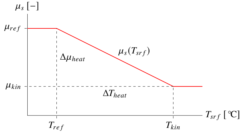
Figure 4.7: Piecewise linear dependence of friction on surface temperature cf. equation (4.18). In this case \Delta\mu_{heat} is negative, resulting in a decreasing coefficient of friction.
