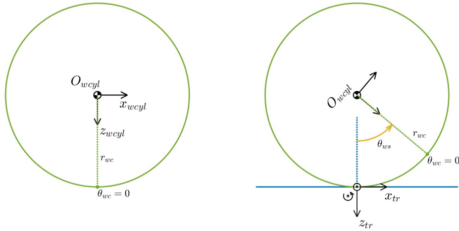
Figure 3.7: Left: definition of cylindrical coordinates (\theta_{wc}, y_{wc}, r_{wc}) on a wheel for wheel out-of-roundness. Right: rotation by the wheelset pitch angle \theta_{ws} .
