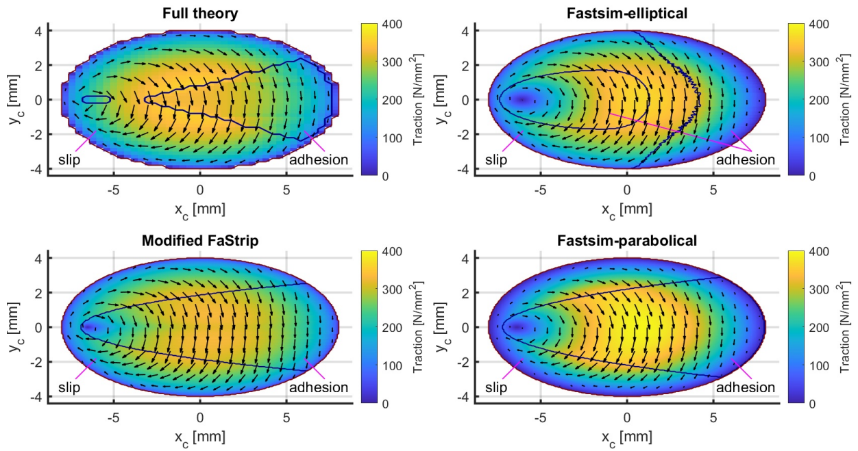
Figure 5.18: Tangential tractions in a steady state rolling problem with large spin. Top-left: results for the CONTACT (half-space) algorithm on a 40 \times 40 grid. Bottom, right: results for FaStrip and for Fastsim with elliptical and parabolical traction bounds, computed on 200 \times 200 grids.
