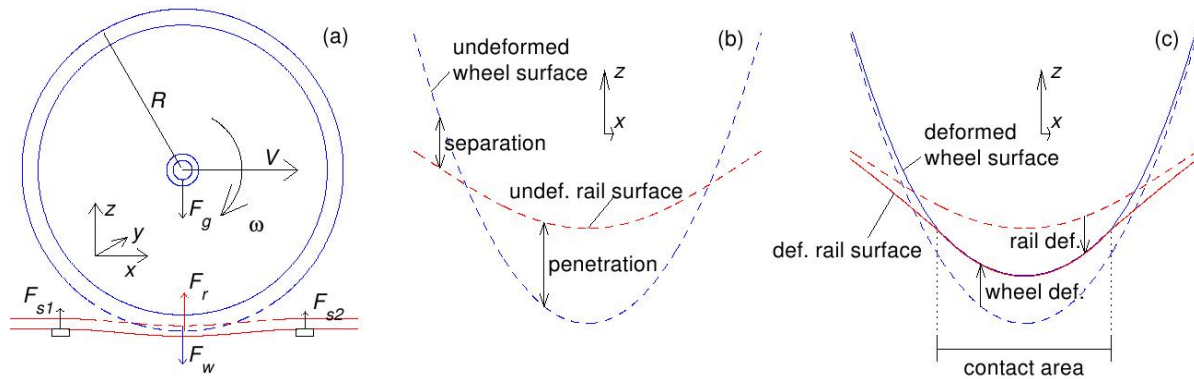
Figure B.2: Illustration of the wheel-rail contact problem [70]. (a): overall geometry. (b): wheel and rail geometries in so-called undeformed states. (c): wheel and rail geometries in the deformed state with corresponding deformations and contact area. Note: graphs (b) and (c) are stretched vertically.
