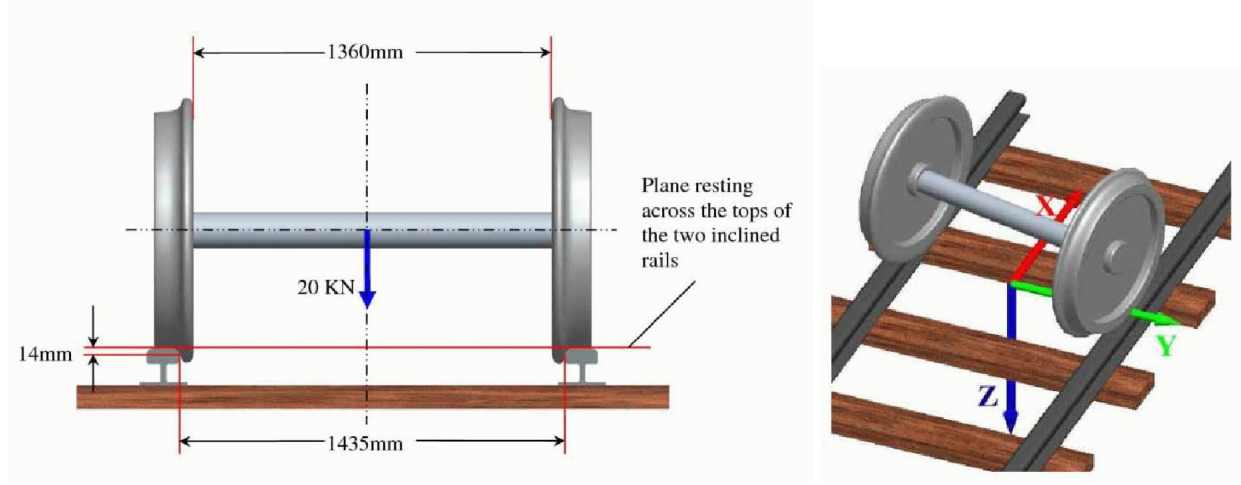
Figure 5.8: Illustration of the simple wheelset model used in Manchester benchmark simulation Case A [41].
