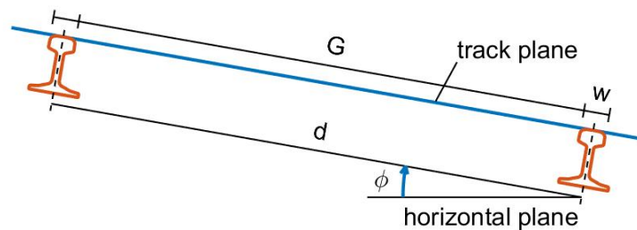
Figure 3.1: Track viewed in world-fixed coordinates, illustrating rail distance d , rail width w , gauge width G , and track inclination (track cant, elevation) angle \phi (adapted from [40]).
