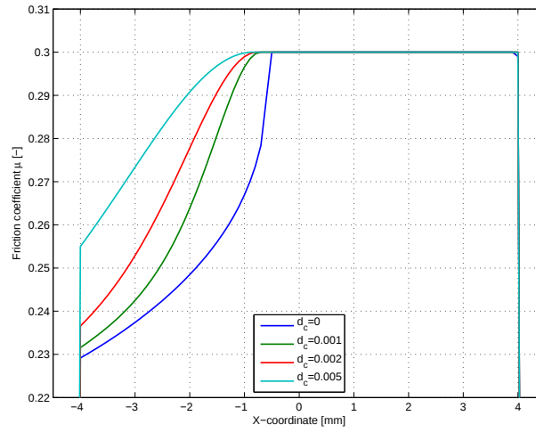
Figure 4.8: Typical effect of friction memory (equation (4.19)) on the friction coefficient \mu : gradual instead of abrupt change of \mu(\mathbf{x}, t) .
