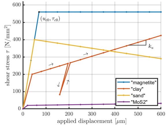
Figure 5.17: Shear stress curves computed by CONTACT for several compounds, mimicking the results of Hou et al. [10, Fig. 4].
