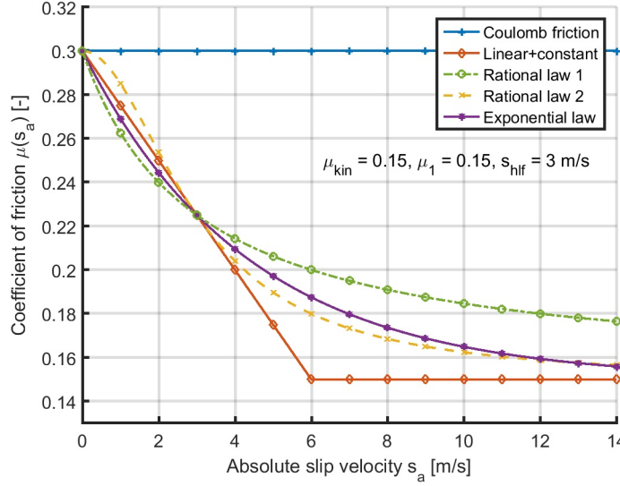
Figure 4.6: Dependence of friction coefficient \mu on absolute slip velocity s_a for the friction laws of equations (4.14)–(4.17).
