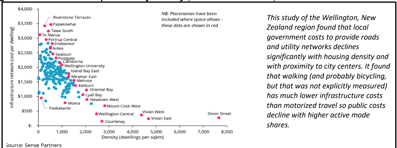
Figure 11 Road and Pipe Costs by Density (Sense Partners 2024)
