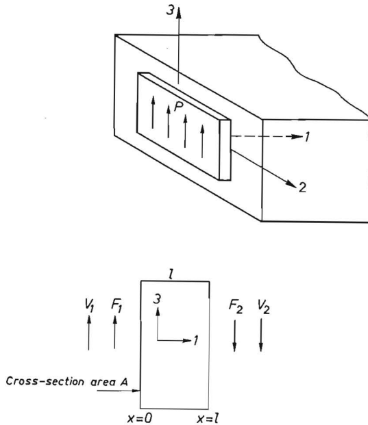
Fig. 4.1. Thickness-shear transducer.
