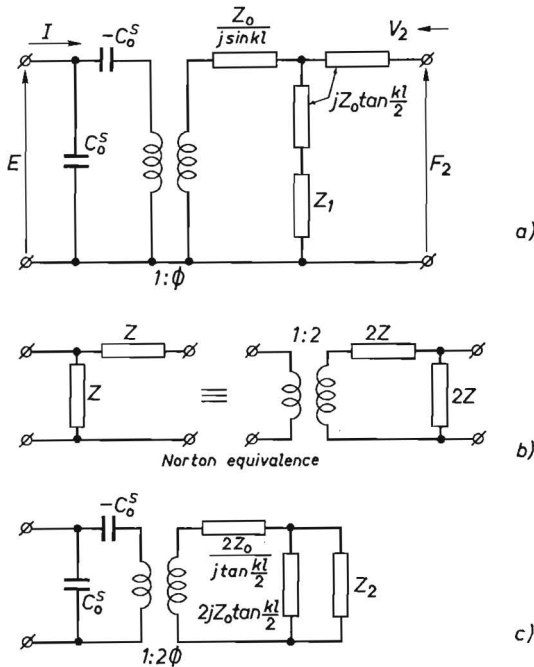
Fig. 4.3. The Norton equivalence is used to transform the circuit a (with Z_1 = 0 ) into that of c .
