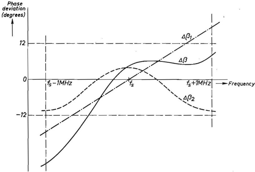
Fig. 2.5. Example of delay-line-phase response meeting the requirements. \Delta\beta_1 = odd component, \Delta\beta_2 = even component, \Delta\beta = total deviation, f_s = colour-subcarrier frequency.
