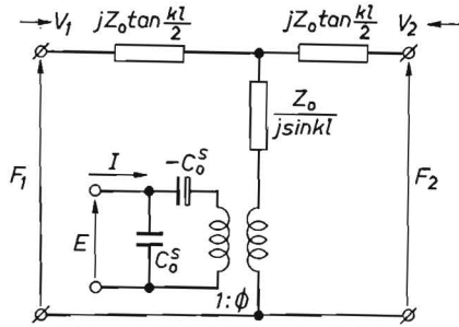
Fig. 4.2. Equivalent circuit for thickness-shear transducer.
