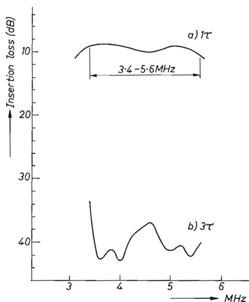
Fig. 3.7. Insertion-loss vs frequency curves of PAL delay line; (a) main signal ( 1\tau ) signal, (b) 3\tau reflection.
