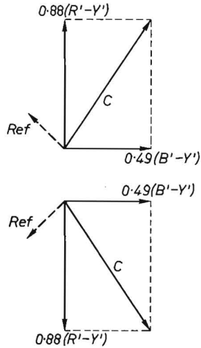
Fig. 2.1. Phasor diagram of the PAL chrominance signal on two consecutive lines.
