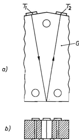
Fig. 3.1. PAL delay line. (a) T_1, T_2 : transducers, G : glass propagation body. (b) In this view the transducers are omitted; the shaded areas represent electrode layers.
