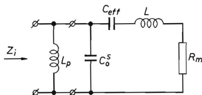
Fig. 4.6. Approximate circuit for unbacked thickness-shear transducer bonded to medium with acoustic impedance \zeta Z_0 ; R_m = \zeta a , L = \frac{\pi}{2} \frac{a}{\omega_a} , C_{eff} = \frac{2 C_0^S}{\omega_a \pi a C_0^S - 2} ; C_{eff} is the series equivalent of -C_0^S and C .
