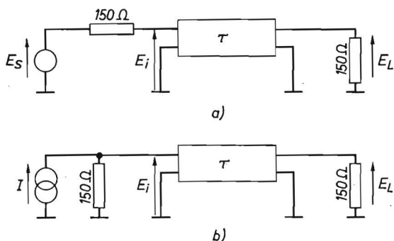
Fig. 5.2. Definition of phase delay.
