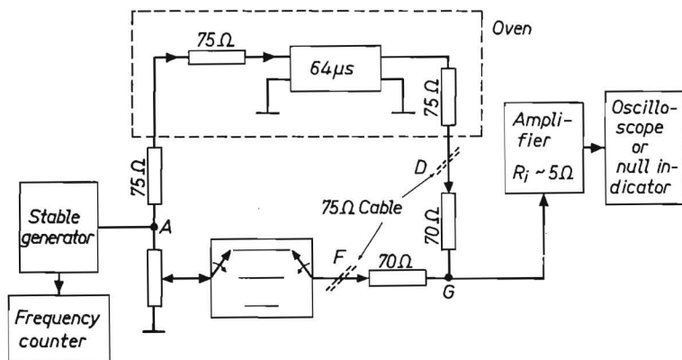
Fig. 5.4. Measurement of phase-delay variation with temperature.
