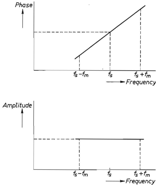
Fig. 2.3. Idealized-network response.
