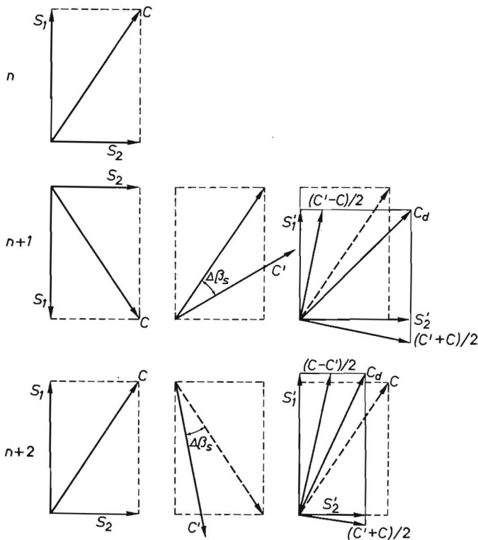
Fig. 2.4. Delay-line-phase-response error \Delta\beta_s at subcarrier frequency. First column: input signal, second column: delayed signal, third column: summation and subtraction; chrominance after detection is represented by C_d .
