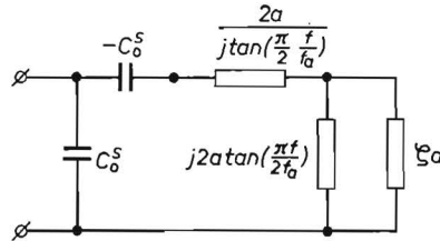
Fig. 4.5. Equivalent circuit of unbacked thickness-shear transducer bonded to medium with acoustic impedance Z_2 = \zeta Z_0 .
