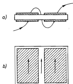
Fig. 3.2. Transducer. View (a) shows schematically the connection of the electrodes; shaded areas represent electrodes; the arrows indicate the direction of polarization.
