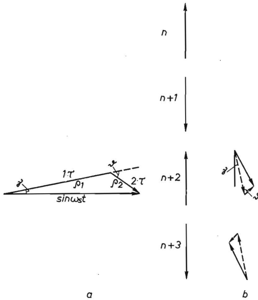
Fig. 2.6. PAL decoding process resulting from the employment of a delay line having 2\tau reflections.
