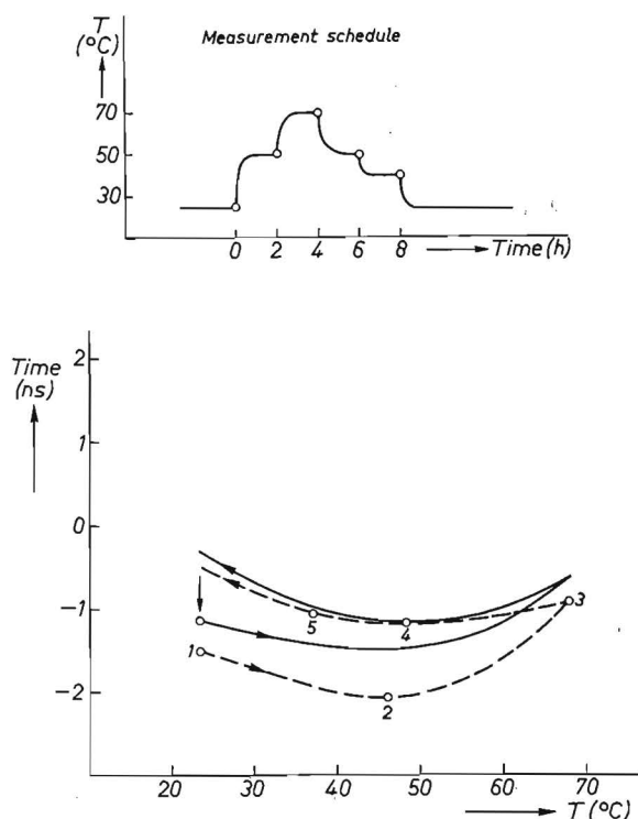
Fig. 3.8. Phase-delay-time vs temperature curves measured on two consecutive days; ----- first day, ————— second day.
