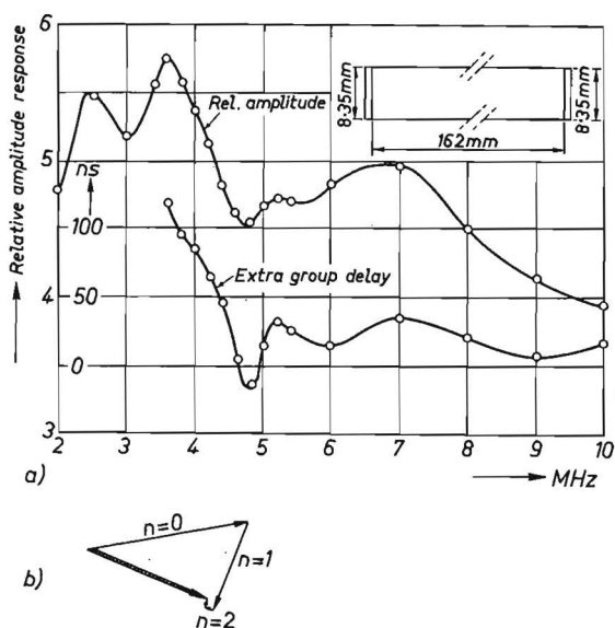
Fig. 4.11. Propagation of quasi shear-vertical waves in a plate. Rays for which n \leq 6 have been included in the computations; n is the number of reflections which a ray suffers between sending and receiving transducers. Plate material: glass 239 ( V_s = 2.54 km/s, \nu = 0.23 ). Plate and transducer dimensions: as in fig. a.
