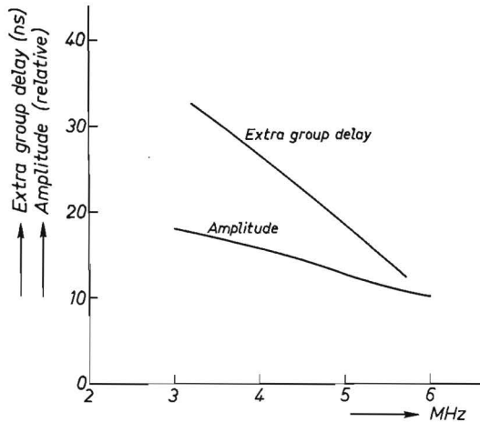
Fig. 3.5. Calculated group delay and amplitude response of delay line having unbonded cross-section. Shear-wave velocity in propagation medium (glass 239): 2.54 \text{ km/s} , length of propagation medium: 160 \text{ mm} , transducer radiating areas: 10 \times 12 \text{ mm}^2 .
