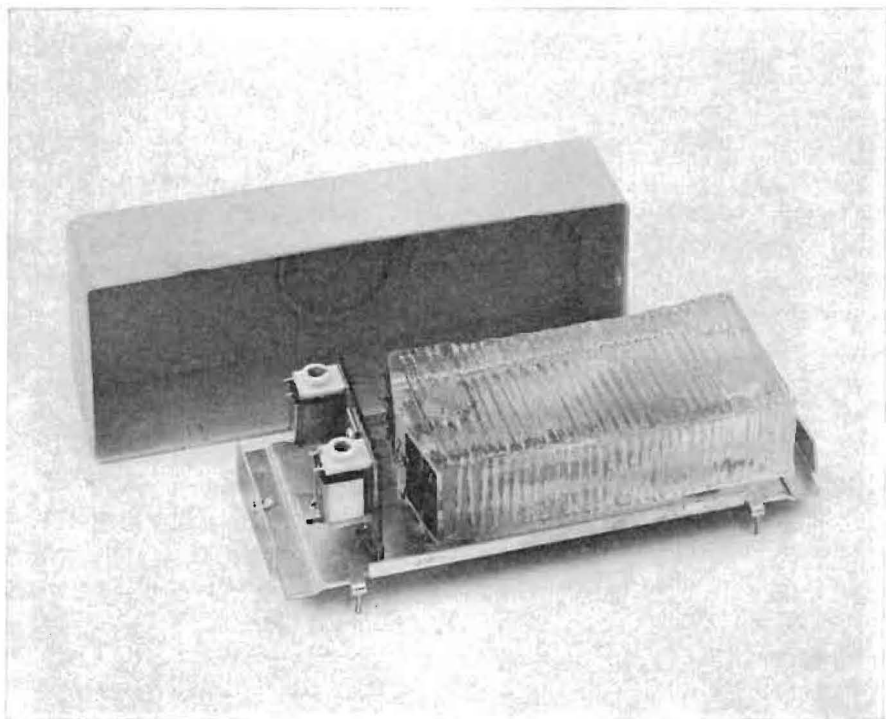
Fig. 3.4. Finished delay line; cover removed.
