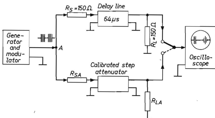
Fig. 5.1. Block schematic arrangement for insertion-loss measurements; R_{LA} = image impedance of attenuator.
