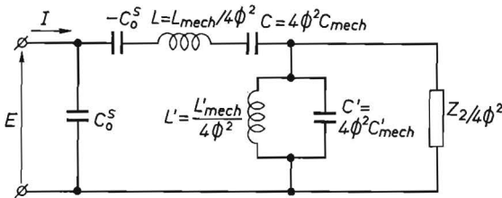
Fig. 4.4. Approximate circuit for unbaked thickness-shear transducer bonded to medium with acoustic impedance Z_2 ; all elements transformed to electrical side. Approximations are best for frequencies around f_a = v^D/2l .
