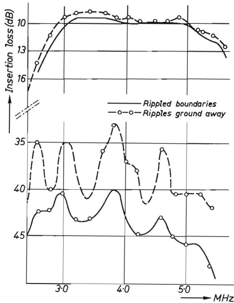
Fig. 4.12. Measured effect of rippling.
