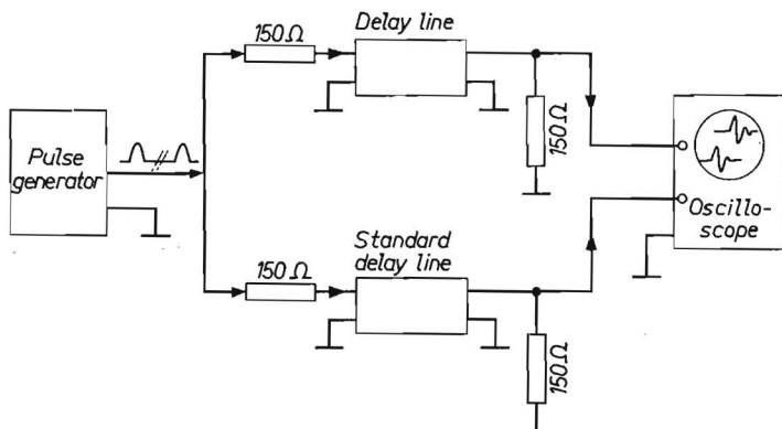
Fig. 5.5. Coarse group-delay measurement.
