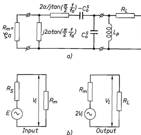
Fig. 3.6. Loss caused by reflections.
