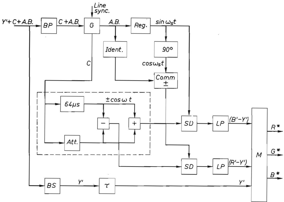
Fig. 2.2. Block diagram of decoder circuit of PAL-d receiver.
