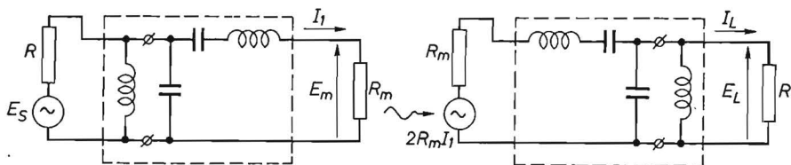
Fig. 4.7. Transducer-pair representation.
