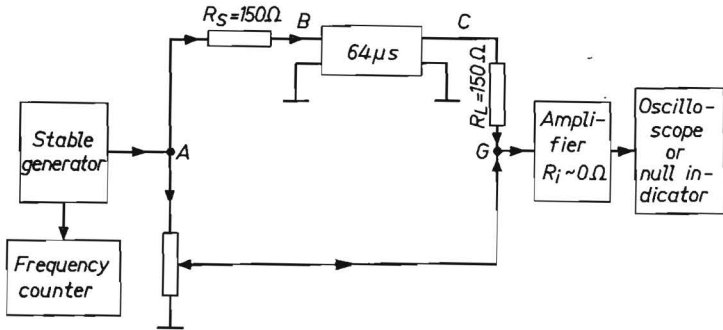
Fig. 5.3. Block schematic arrangement for phase-delay measurements.
