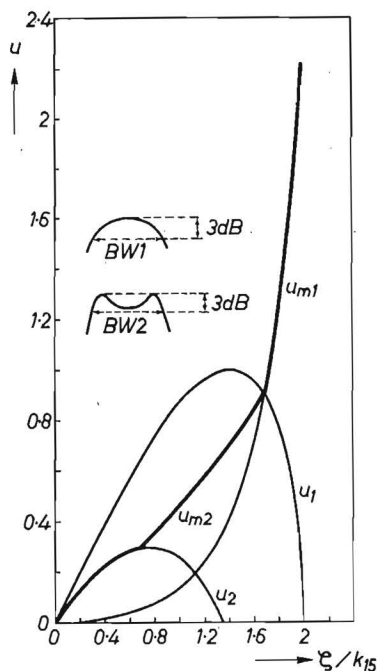
Fig. 4.8. Approximate analysis of transducer-pair response. For a given value of \zeta/k_{15} , maximum bandwidth is obtained if u lies on the fat curve u_2 - u_{m2} - u_{m1} ;
