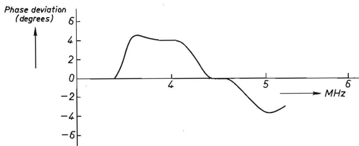
Fig. 3.9. Measured deviation from ideal response.
