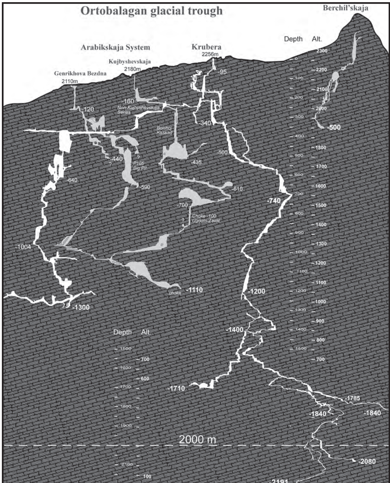
Figure 3: Combined cave profile along the axis of the Ortobalagan valley. Krubera Cave is shown in white, other caves in light grey.
