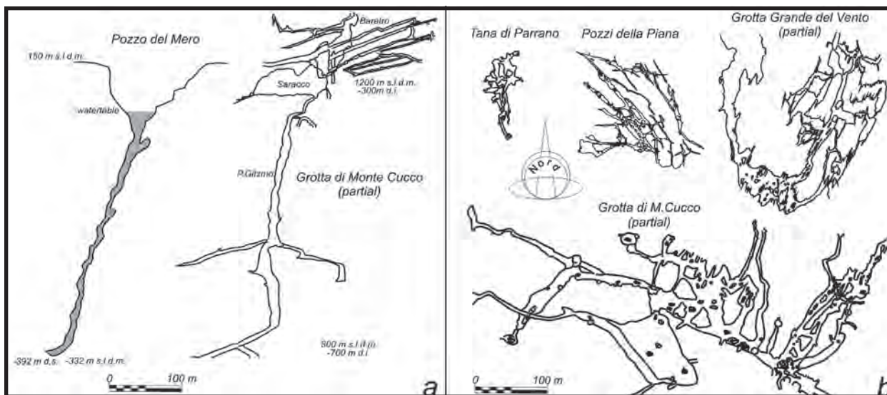
Figure 3: Patterns of caves in central Italy. a – cross section of the Pozzo del Merro compared with the deeper part of the Monte Cucco Cave; b – plan view of major hypogenic caves compared with a few branches of the Grotta Grande del Vento (Frasassi) and Monte Cucco Caves.
