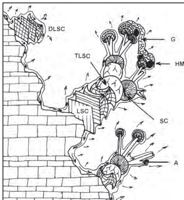
Figure 2: Diagram showing cross section of wall rock with saturated seepage film, which thins outward. The effect of evaporation is greatest on thin films with little through flow, creating a series of closely spaced microenvironments in which a succession of minerals and crystal morphologies evolve: length-slow calcite (LSC), deformed length-slow calcite (DLSC), twinned and deformed ball of length-slow calcite (TLSC), balls of calcite showing split-crystal growth (SC), aragonite prisms (A), hydromagnesite (H) and gypsum (G).
