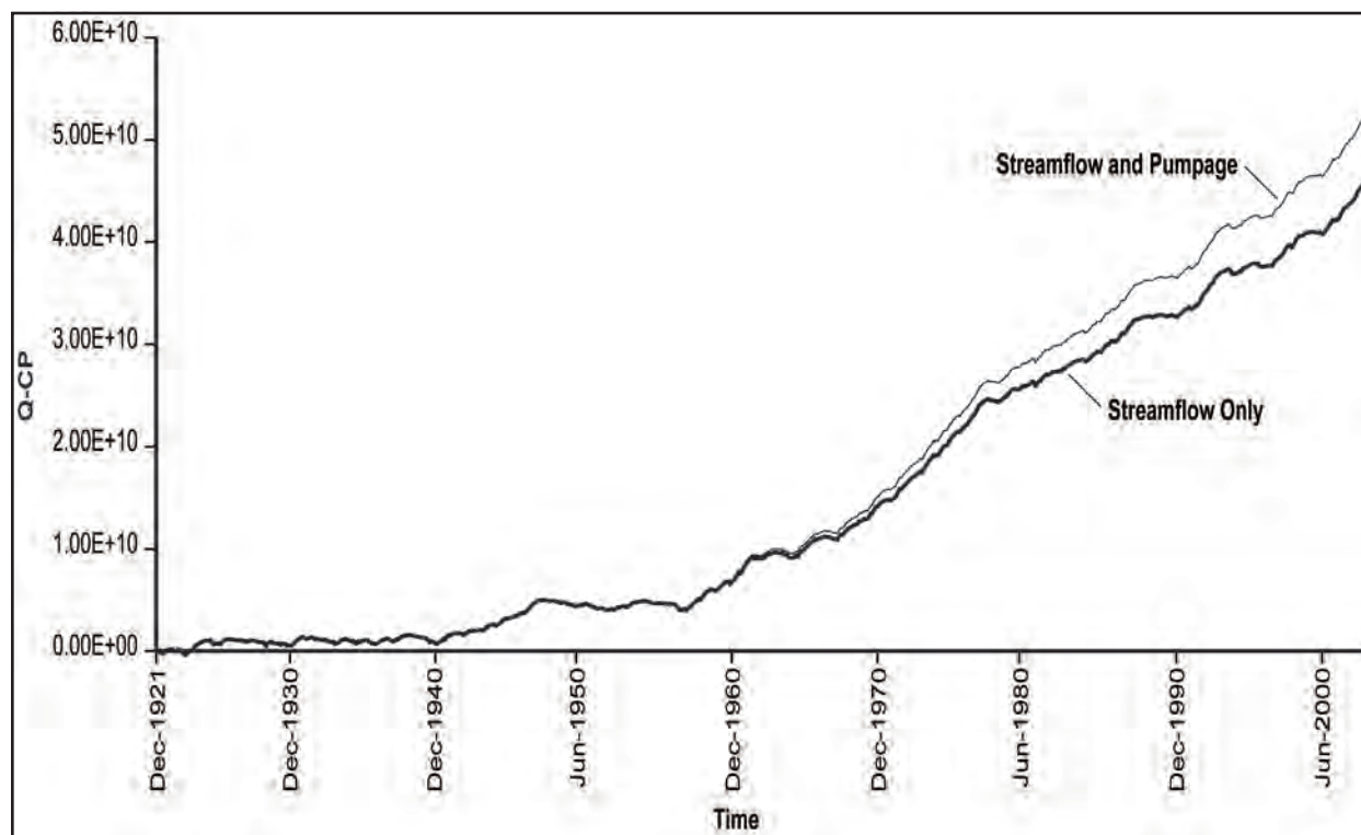
Figure 3: Cumulative Barton Springs flow (and pumpage from the Barton Springs segment of the Edwards Aquifer) less cumulative estimated recharge from precipitation. Note the departure occurring after 1960 that is attributed to urbanization.
