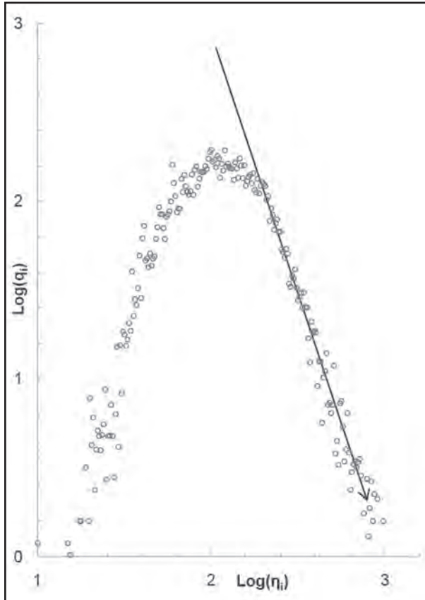
Figure 3: Histogram of LME number distribution with logarithmic interval binning of 2 % of size (cm). The apparently linear power-law range was chosen to be 184 to 591 cm for the estimation of the fractal dimension of the cave. The peak is at the nominal proper modulus (1.1 m) of the cave.
