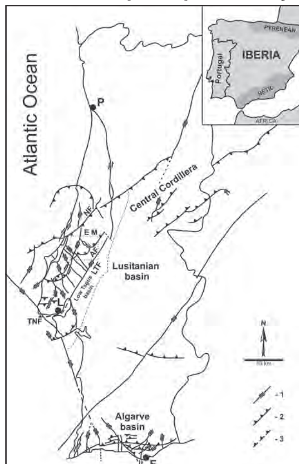
Figure 1: Map of structures active in Portugal during the Alpine collision (with minor modifications, from Ribeiro et al, 1990). 1 - Strike-slip faults; 2 - thrust faults; 3 - Probable thrust faults. NF - Nazaré fault; AF - Arrife fault; LTF - Lower Tagus fault; TNF - Tagus neck fault; EM - Estremenho massif. P - Oporto; L - Lisbon; F - Faro. Dashed square = area represented in Fig. 2.
