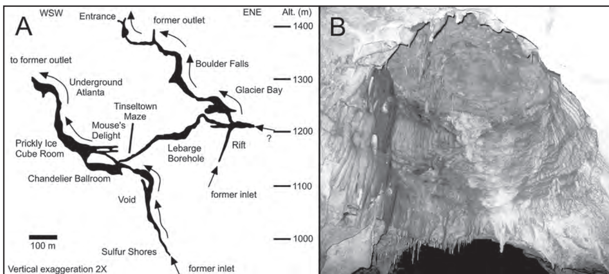
Figure 3: Guadalupe Mountains. A) Simplified profile view through part of Lechuguilla Cave in the Guadalupe Mountains shows the flow paths of ascending fluids (from Palmer and Palmer, 2000); b) typical cupola (~4 m in diameter) in a Guadalupe Mountains hypogene cave.
