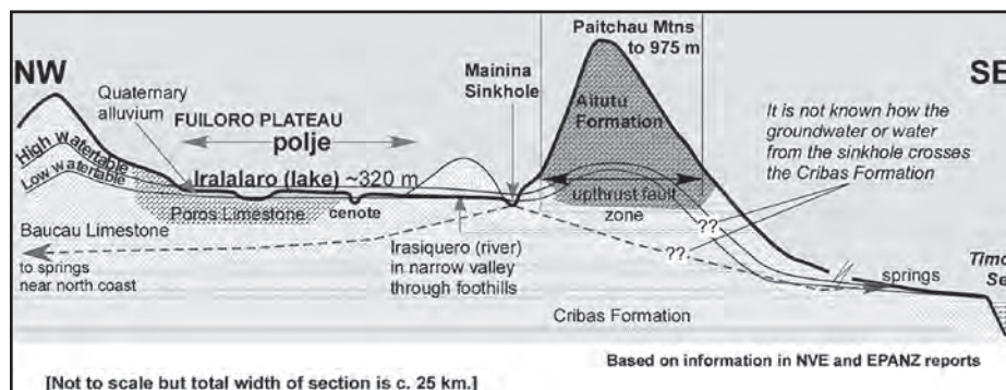
Figure 6: Schematic cross section through Iralalaro (lake) and Paitchau Mountains, Lautem District, Timor Leste.
