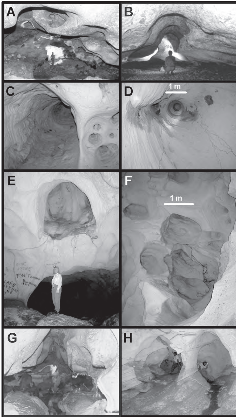
Figure 1: Bedrock dissolutional morphologies, or speleogens, from flank margin caves in the Bahamas and Isla de Mona, Puerto Rico. These dissolutional features are nearly identical to those described in Klimchouk (2007) as being produced solely by confined hypogenic conditions in karst aquifers. (A) Rising chain of cupolas, Cueva del Agua Punte los Engelses, Isla de Mona. Compare to Plates 6C and 6D in Klimchouk (2007). (B) Ceiling channel, Cueva del Agua Sardinera, Isla de Mona, Puerto Rico. Compare to Plates 6G and 7A in Klimchouk (2007). (C) Domepit (sensu Klimchouk, 2007), Cumulous Cave, Crooked Island, Bahamas. Ruler in right center is 10 cm long for scale. Compare to Plate 9J in Klimchouk (2007). (D) Cupola with outlet, Hamiltons Cave, Long Island, Bahamas. Compare to Plate 9D in Klimchouk (2007). (E) Large Cupola, Hatchet Bay Cave, Eleuthera Island, Bahamas. Compare to Plate 6D in Klimchouk (2007). (F) A variety of ceiling cupolas, Hatchet Bay Cave, Eleuthera Island, Bahamas. Compare to Plates 6B, 6C, 6I, 9B, and 11A in Klimchouk (2007). (G) Fissure and rift-like passage, Cueva del Agua Sardenra, Isla de Moan, Puerto Rico. Compare with Plates 5H and 5I in Klimchouk (2007). (H) Bedrock partition, Goat Cave, Long Island, Bahamas. Compare to Plates 12E and G in Klimchouk (2007).
