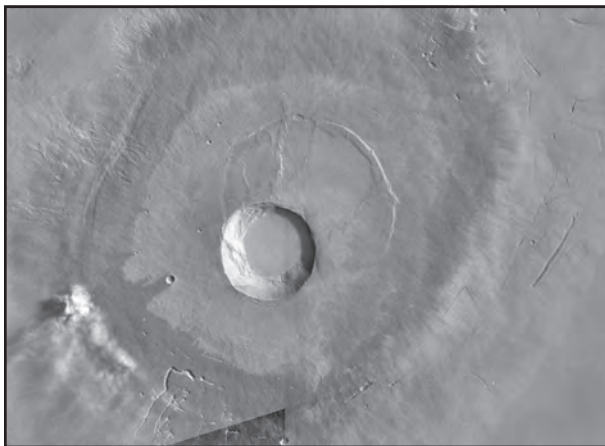
Figure 12: Caldera collapse pit at the summit of one of the large volcanoes on the Tharsis plateau. Image from NASA (Courtesy of Windows to the Universe, http://www.windows.ucar.edu ).
