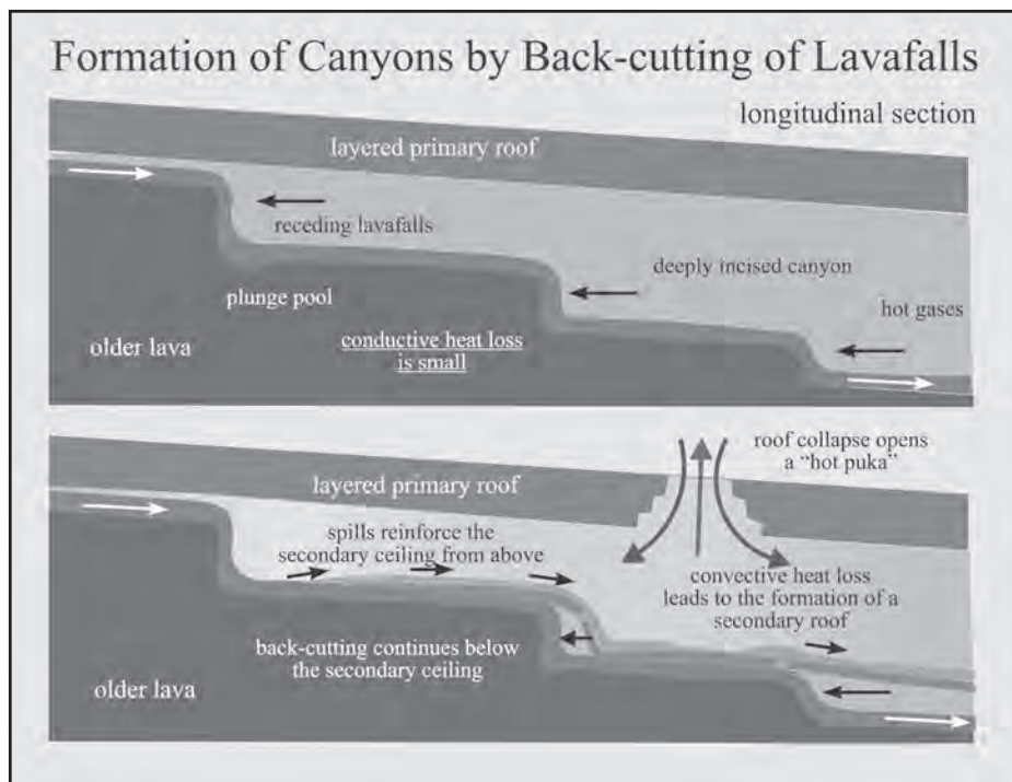
Figure 3: Longitudinal section of an evolving lava tunnel. Top: Erosional enlargement of the underground canyon by backcutting lavafalls. Bottom: Upon static failure and partial collapse of the primary roof a skylight (puka) opens up, allowing cold air to enter the tunnel, freezing an internal secondary roof below which erosional enlargement can continue. Spills from uphill or through holes reinforce the secondary roof.
