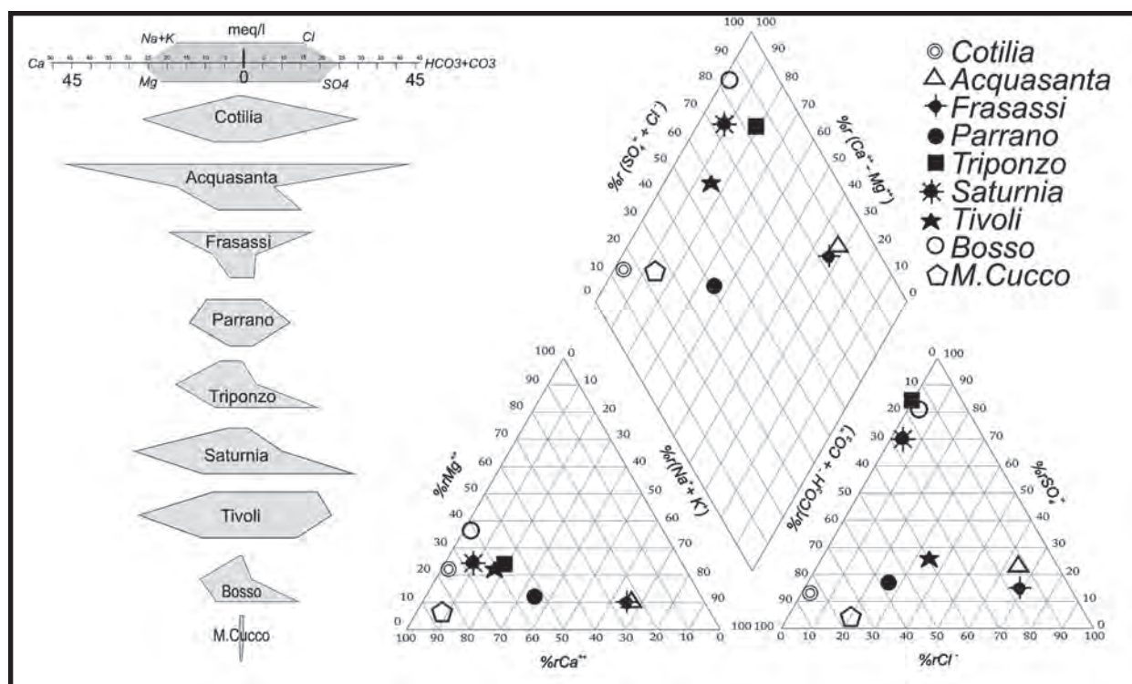
Figure 2: Geochemistry of the karst waters in central Italy. Stiff diagrams on the left and Piper diagram on the right. Location of the springs is shown in Figure 1.
