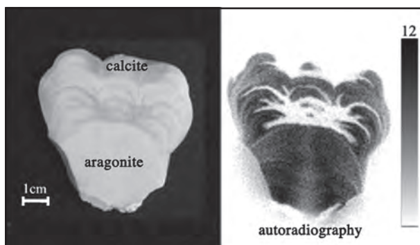
Figure 1: Corallite speleothem from Aranzadi Gallery (Pierre Saint-Martin, Pyrenees). Left : polished section with aragonite (white) and neoformation calcite (grey). Right : autoradiography after 13 days showing radioactive aragonite.
