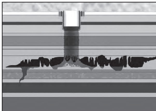
Figure 1-6: Drilling intersects cave, fluids enter cave system.
