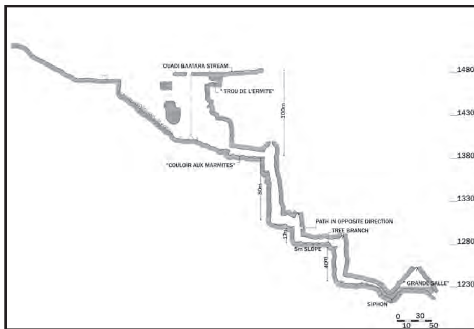
Figure 1: Section of Baatara pothole: dimensions are in meters including elevation above sea level in Y axis (source: Spéléo-Club du Liban archives).
