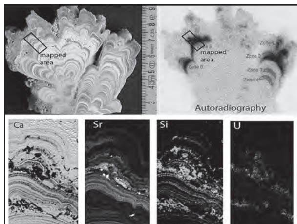
Figure 3: Corallite speleothem in Mechta Cave, Tageran (Baikal, Russia). Top: polished section (left) and autoradiography (right) showing the radioactive areas (in black). The rectangle indicates the area analyzed by \mu -XRF. Bottom: \mu -XRF mapping of Ca, Sr, Si and U. There is a reverse correlation between Ca and Si (opal), and a positive correlation between Si (opal) and U.
