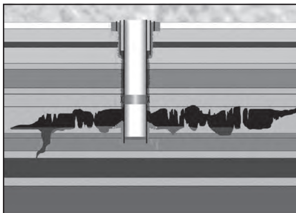
Figure 1-9: Cement first stage at base of cave.
