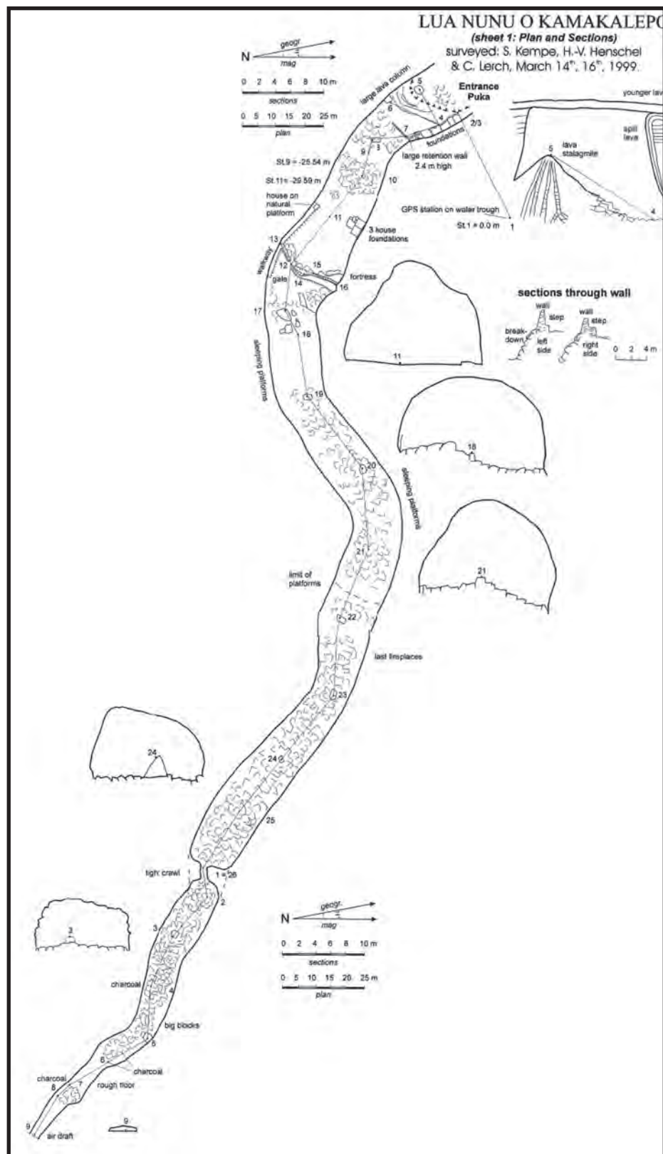
Figure 2: Map of Lua Nunu o Kamakalepo Mauka Cave. Note archeological details.
