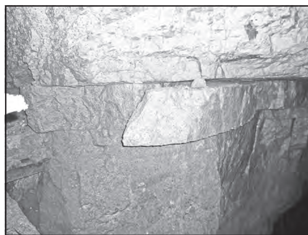
Figure 3: Unstable limestone block on the west side of the stairway.
