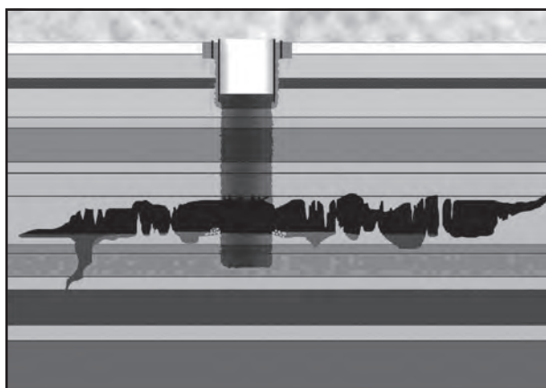
Figure 1-7: Drill into competent formation below cave.
