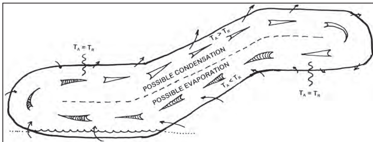
Figure 4: Rayleigh-Benard convection in a closed cave. The degree of heat exchange depends on the difference between the temperature of the cave air ( T_A ) and that of the bedrock away from the passage wall ( T_R ).
