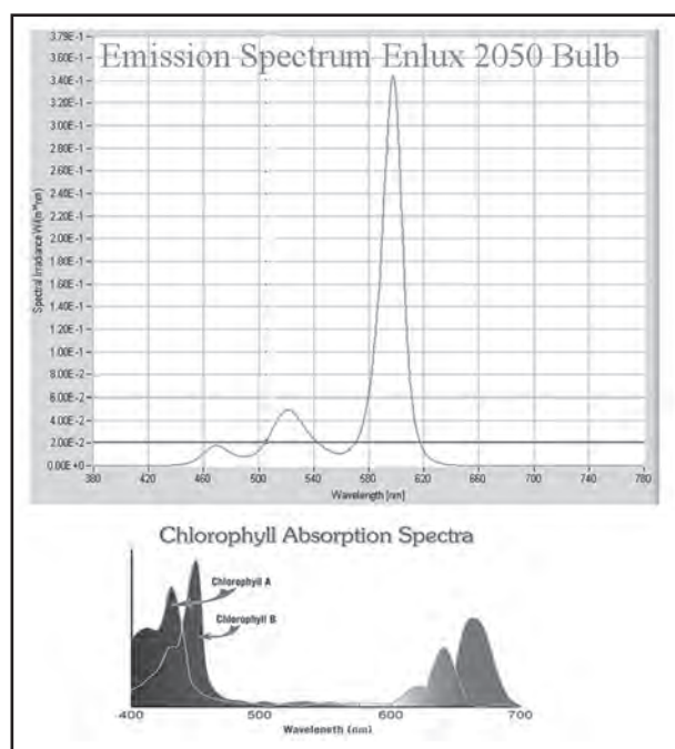
Figure 6: Emission spectrum of the EnLux W2050 bulb (top) and the absorption spectra of Chlorophyll A and B (bottom). They are aligned with each other along the wavelength axis. Note that most of the light from the EnLux bulb occurs in wavelengths that are not very effective at driving photosynthesis. This is a light designed to not promote plant growth.
