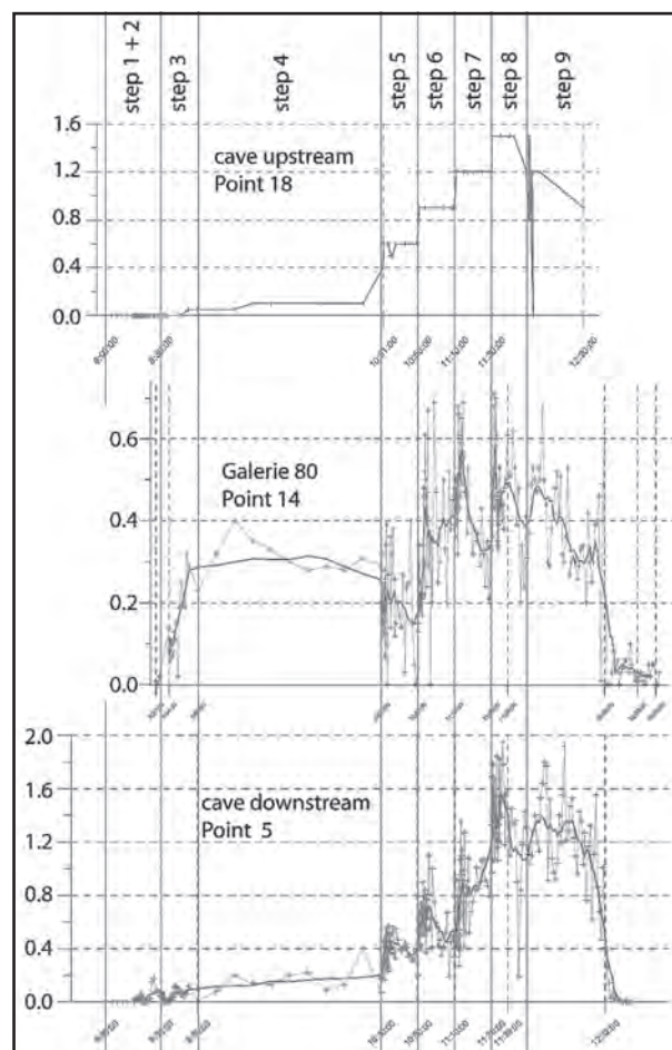
Figure 3: Draft velocity in m/s measured at three locations in the cave.
