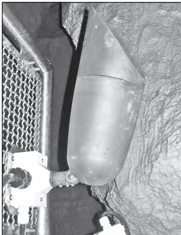
Figure 4: Large Hadco bullet fixture mounted to the railing grille with a plastic junction box. Note the angled snoot on the top to direct the light and prevent glare.
