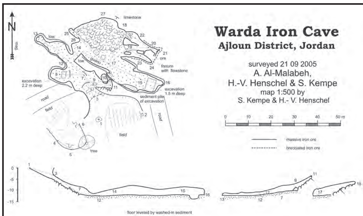
Figure 2: Map and cross-sections of the historic Warda Iron Ore Mine/Ajloun District.
