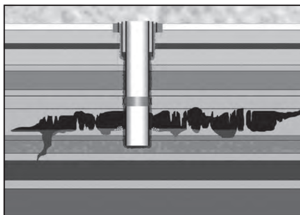
Figure 1-8: Set intermediate casing with external packer.
