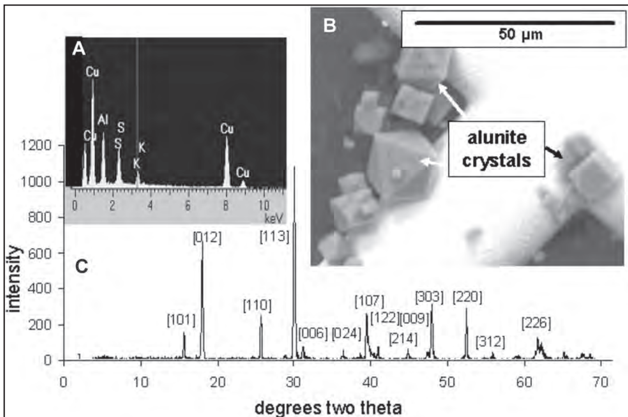
Figure 3: The Kraushöhle alunite is the K-rich endmember. A) the three detectable elements using EDS are Al, S, and K; B) crystals are micron-sized rhombs; C) the XRD pattern of the HF-treated aliquot indicates that alunite is the only crystalline phase.
