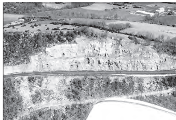
Figure 3: Section in the Bajocian cherty limestone in the Grands Causses (France). We can recognize pockets of clay with chert (dark grey formation), but also pseudo-endokarst under a roof of competent limestone.
