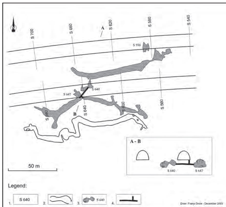
Figure 7: The expressway lay-out with newly discovered caves. 1: profile, 2: cave known before construction accessible from the surface, 3: newly discovered cave accessible from the tunnel, 4: concrete tube connecting newly discovered cave and tunnel.
