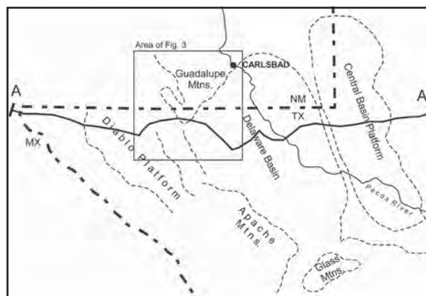
Figure 1: Index Map of the Guadalupe Mountains and vicinity. A – A' is the cross section shown in Figure 4.
