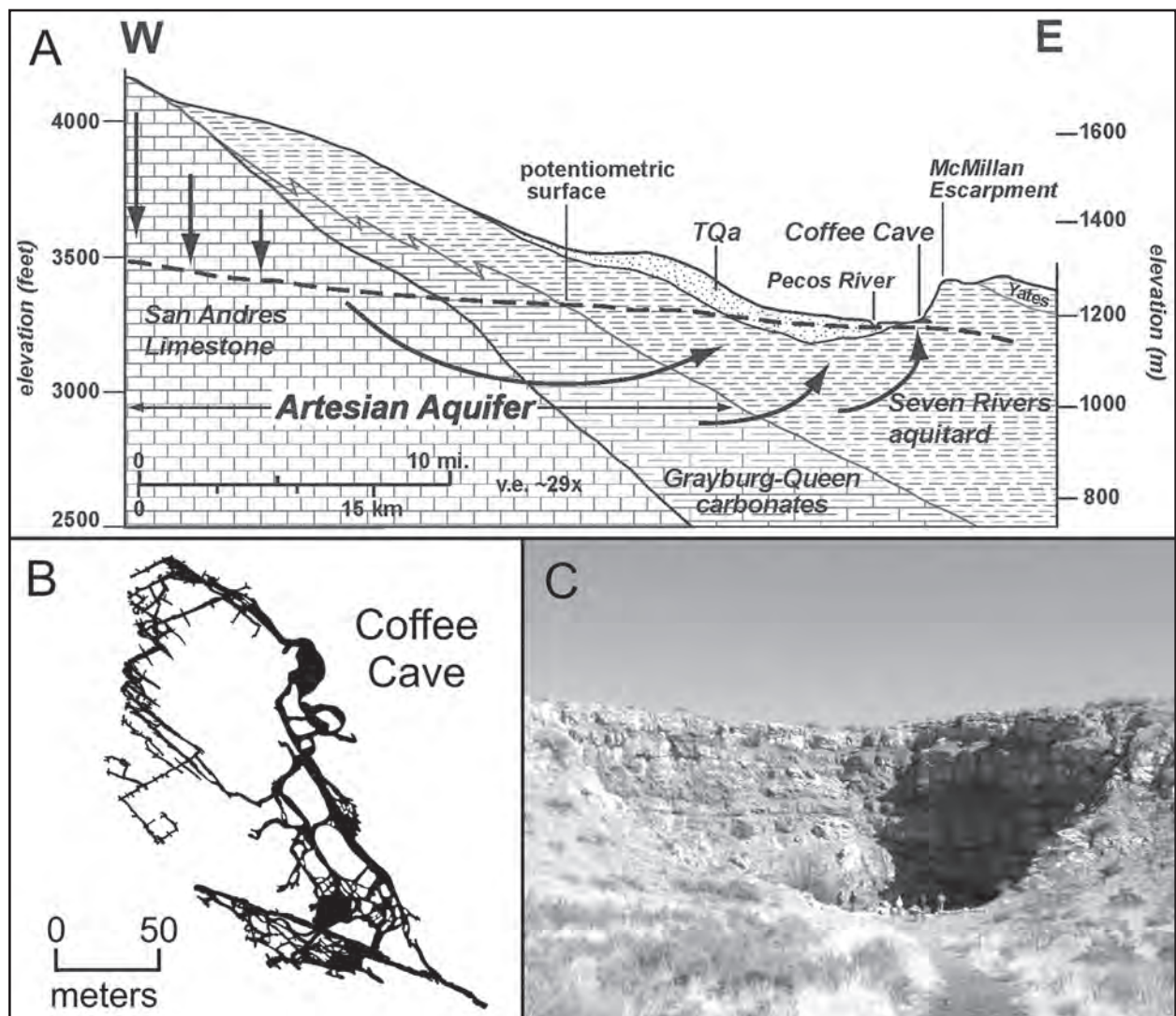
Figure 4: Northwestern Shelf. (A) Hydrostratigraphic section showing relationship between Coffee Cave and the underlying Artesian Aquifer (from Stafford et al., 2008a); (B) Plan view outline map of Coffee Cave showing maze pattern (from Stafford et al., 2008a); (C) Large collapse structure near Roswell, New Mexico. Note people in middle of photo for scale.
