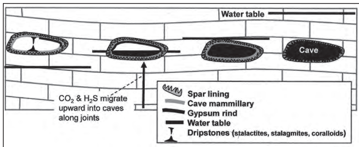
Figure 3: A diagram illustrating the progression of speleothem deposition related to the descending position of the water table. Spar lines cave walls in the phreatic zone below the water table, mammillaries form just below the water table, folia and cave rafts form along the surface of the water table when the water table descends to cave level, replacement gypsum rinds form just above the water table, and speleothems like stalactites and stalagmites form above the water table in the subaerial zone. The small-scale folia and cave rafts are not illustrated.
