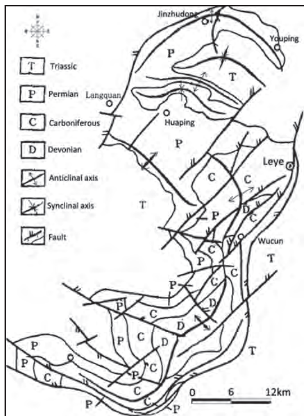
Figure 4: S type geological structure.
