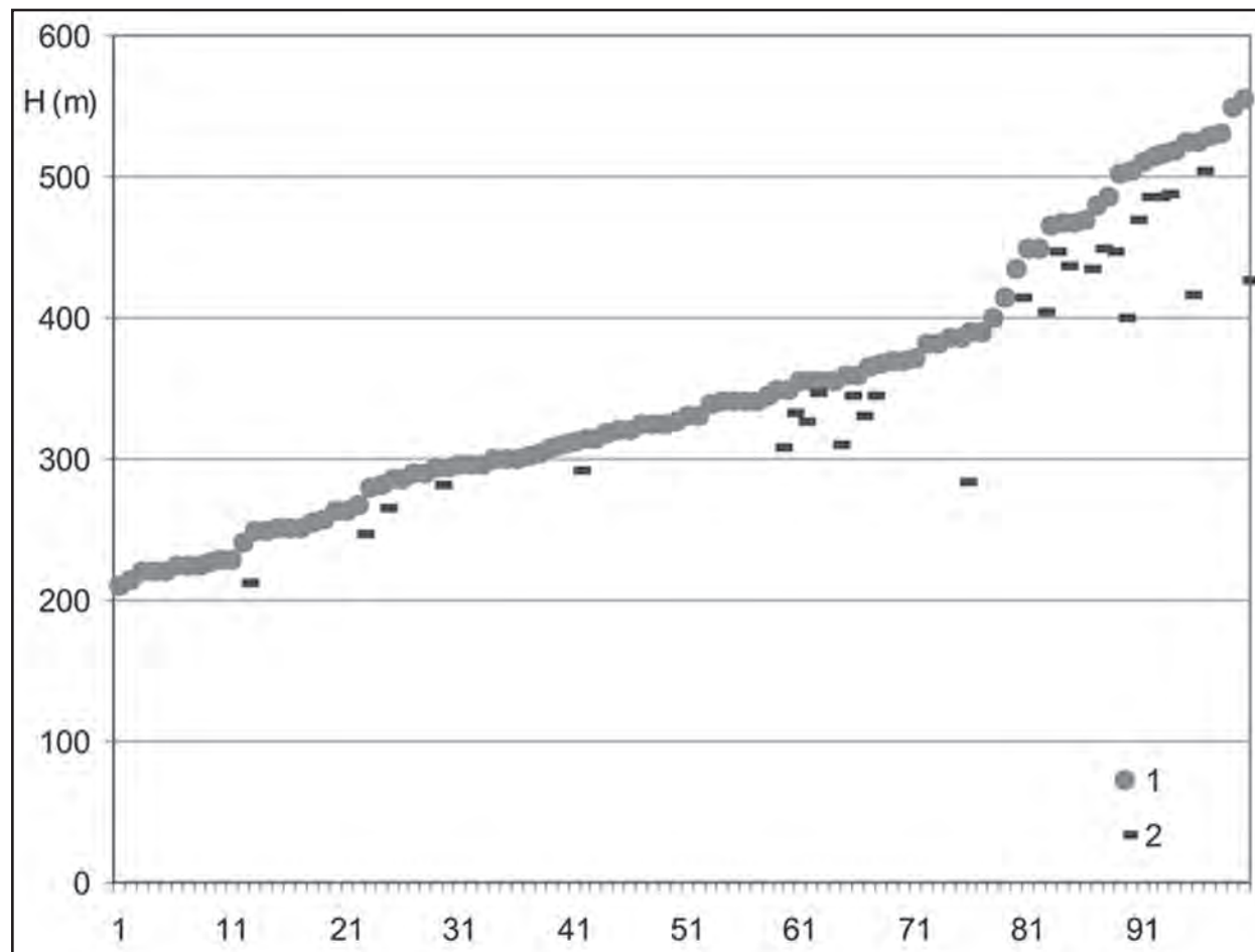
Figure 2: Plot of cave entrance elevations (1) sorted by elevation above sea level (dots), and (2) elevations of lowest points in caves (rectangles), plotted directly beneath their corresponding entrance points. Most caves are too shallow for their deep points to be distinguished on the graph.
