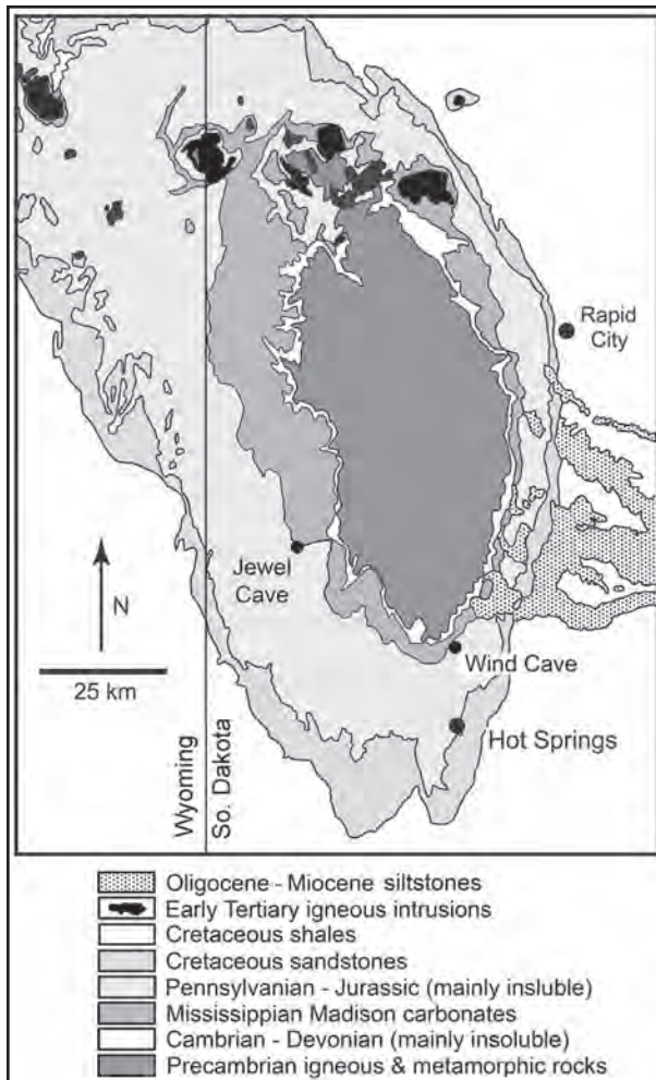
Figure 1: Map of the Black Hills, South Dakota and Wyoming, showing the geologic setting and location of caves.
