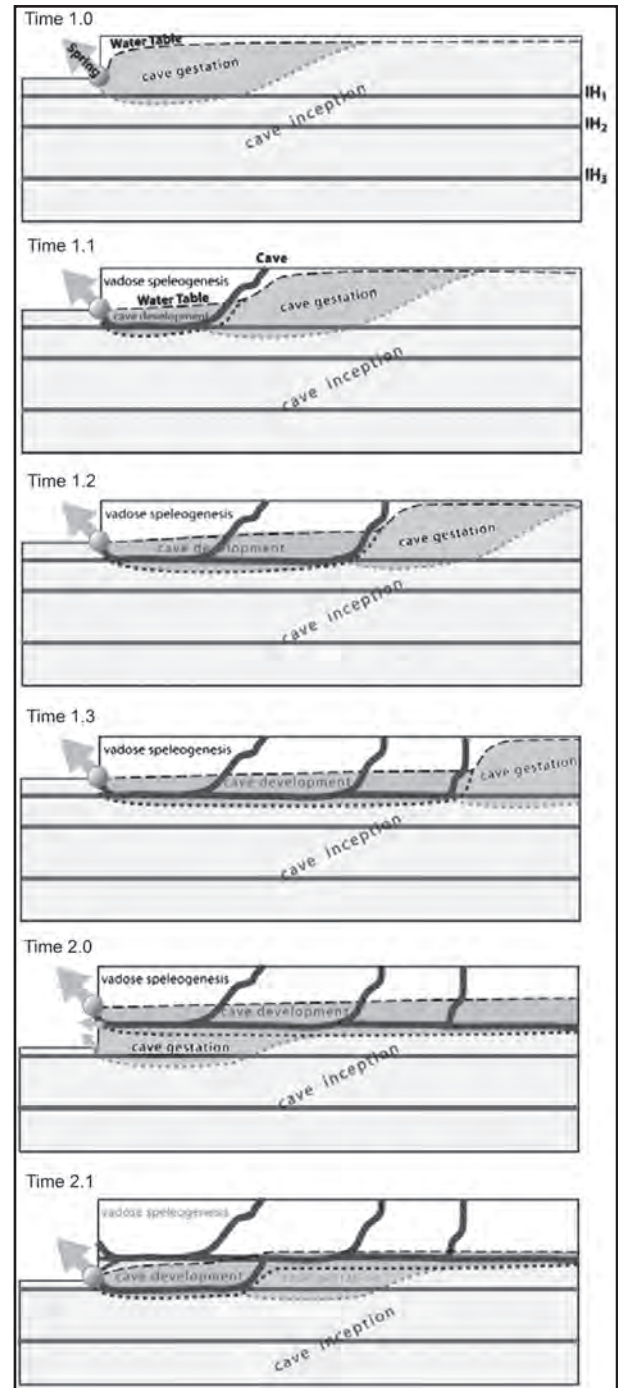
Figure 4: Schematic development of a karst system in time and space (vertical section) with horizontal inception horizons (IH): Different parts of the rock massif are in different karstification zones at the same time. Shortly after a valley incision event (time 1.0 and 2.0) the gestation zone is located near the spring. Karst conduit network begins to develop along the inception horizons within the gestation zone. As a conduit within this zone begins to allow turbulent flow, the water table drops. The gestation zone becomes a cave development zone and a new gestation zone develops upstream. This upstream shift of the gestation and development zones produces typical cave levels.
