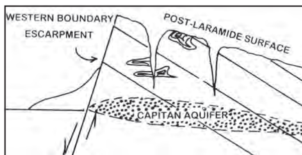
Figure 3b: In the late Miocene to Recent, normal faulting along the Rio Grande Rift elevates the earlier formed erosional surface, resulting in the development of a fresh water lens beneath the mountains.
