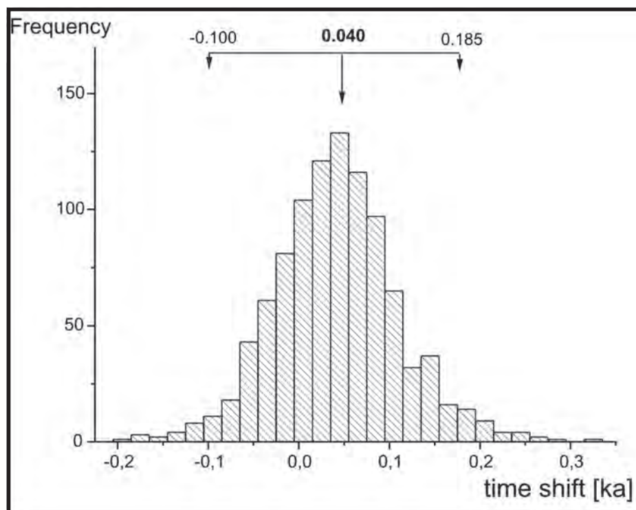
Figure 4: Correlation quality estimation basing on mean record distance as a similarity parameter. Histogram of parameters represented by correlation analyses repeated 1,000 times.
