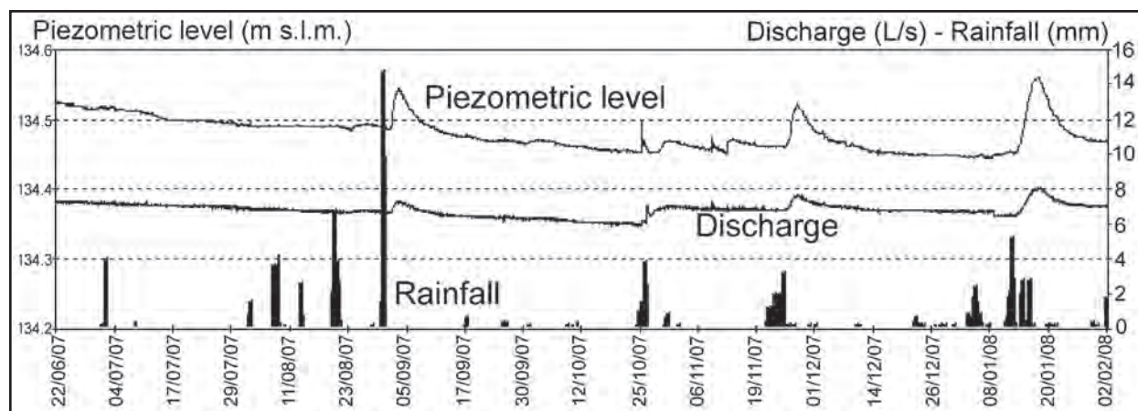
Figure 3: Flow rate, water levels and rainfall in the period June 22, 2007 – February 2, 2008 (piezometer S4).
