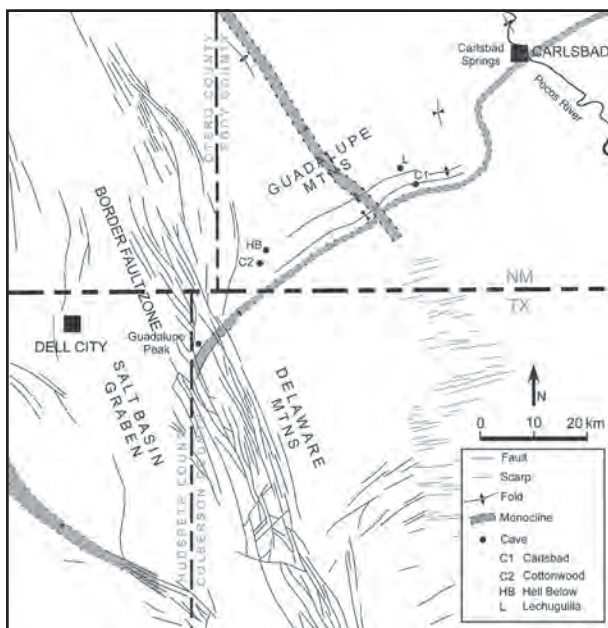
Figure 3: Tectonic map of the Guadalupe Mountains and vicinity with key landmarks and caves. Modified from Hayes, (1964, fig. 24).
