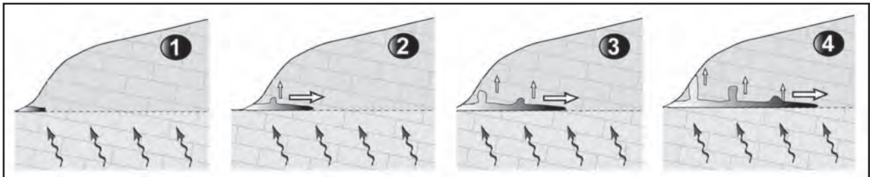
Figure 8: Water table Sulfuric cave. Headwards evolution by condensation-corrosion along the water table, supplied with major sulfuric upwelling along a fracture. Simultaneously, hydrothermalism lifts the hot air, condensation-corrosion occurs, bells and chimneys develop, some finally break through to the surface. The white arrows indicate the direction of cave development (inspired from Cueva de Villa Luz, Mexico).
