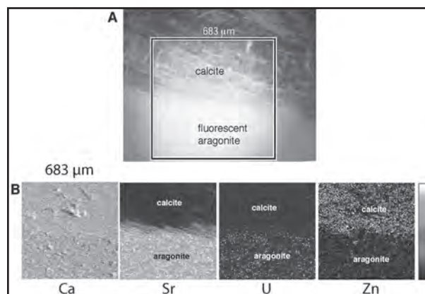
Figure 2: Nuclear microprobe mapping at the contact aragonite-calcite for the corallite sample AR2002 (Pierre Saint Martin, Pyrenees). Sr and U are concentrated in aragonite and Zn in calcite.
