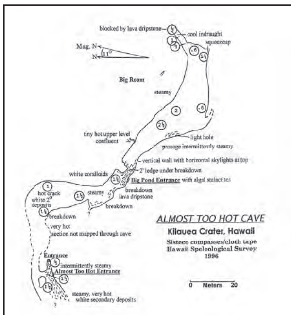
Figure 6: Plan of Almost Too Hot Cave. Ceiling heights are in meters.
