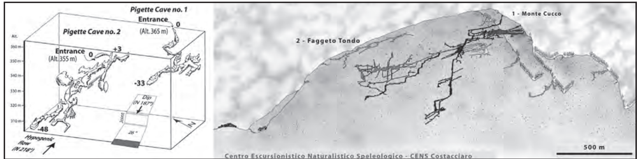
Figure 3: Left: perspective view of the Pigette Caves (France), a 3D multistorey maze cave originating in the phreatic zone by hypogenic upwelling, following structural weaknesses (inclined dip and vertical joints) (sketch by J.Y. Bigot). Right: Monte Cucco system (Italy), probably the deepest hypogene cave system of the world (- 923 m / 31 km), with large shafts of several hundred meters of depth and ramps inclined along the dip of the anticline (Cairolì et al. 1991).
