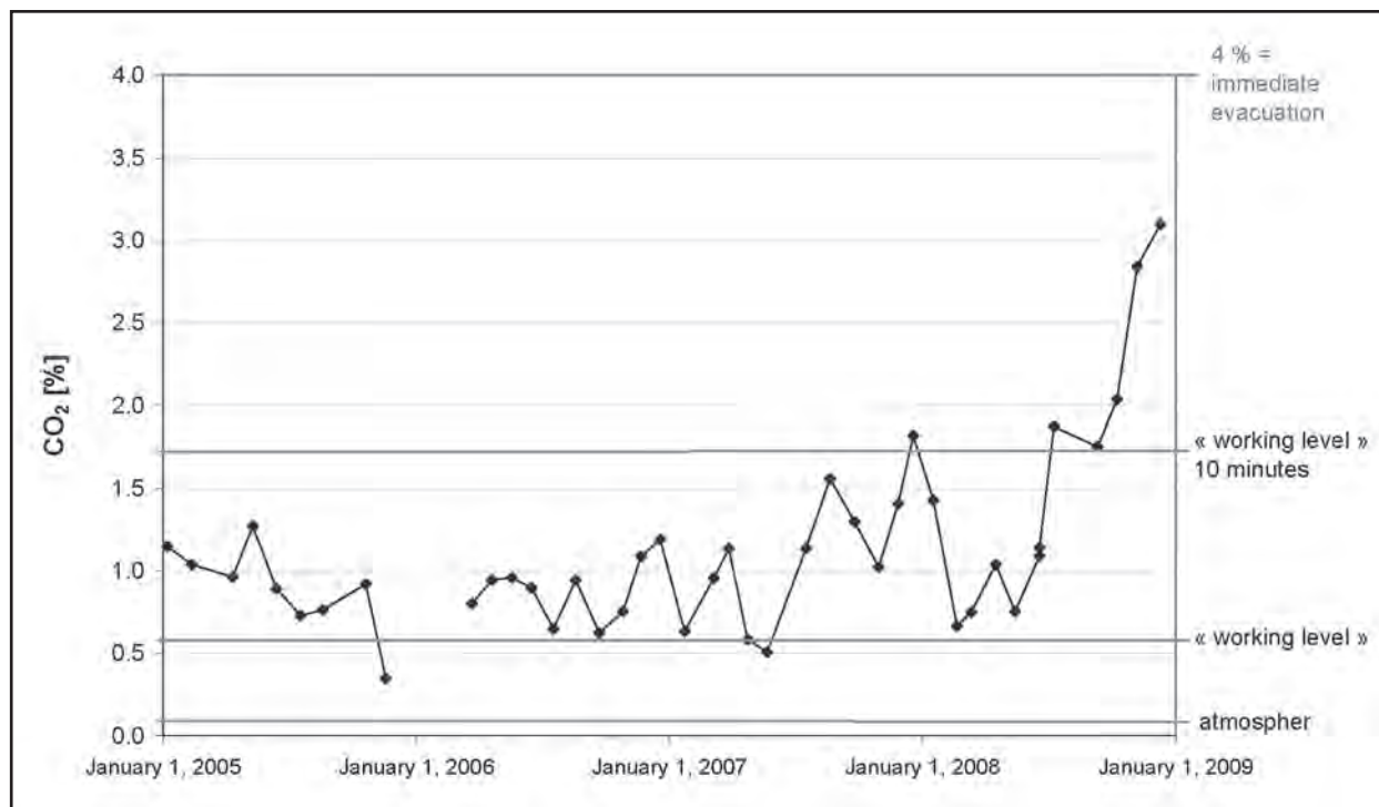
Figure 1: Average CO 2 concentration from 4 different measurement stations in the Milandre Cave between 2005 and 2008. The lowest values are usually observed in between December and March, and the highest values in shortly before. Concentration in 2008 reached very high values.
