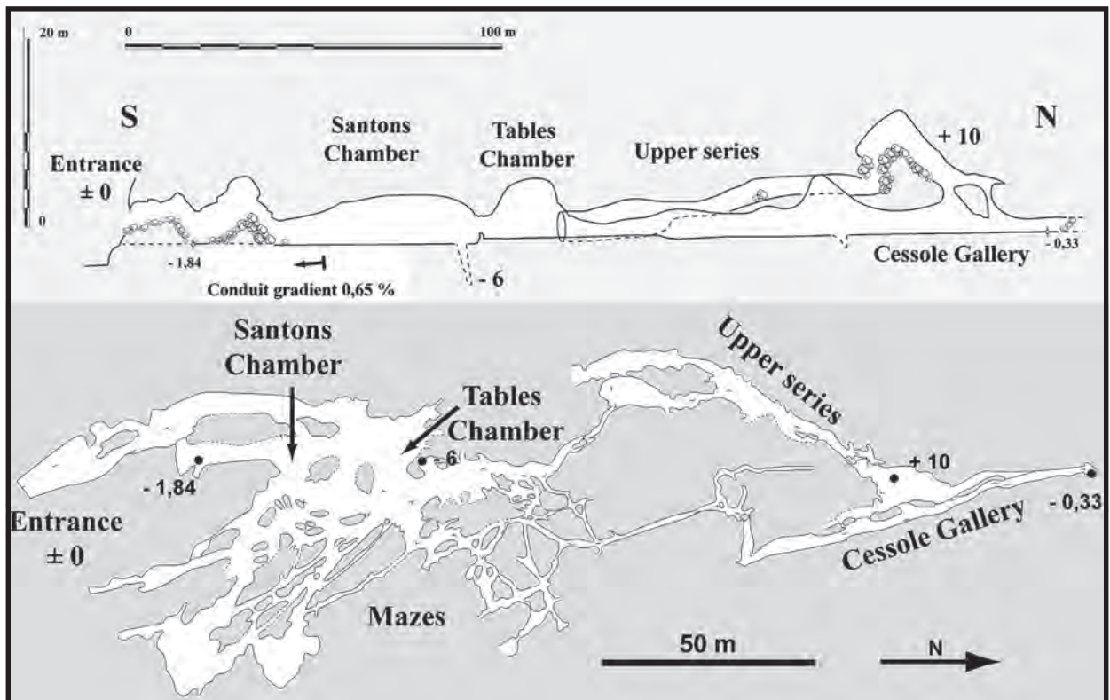
Figure 9: Chat Cave, France. The long profile with very low gradient (0.7%) results from the sulfuric flows. Incipient mazes beside the main drain result from lateral migration of the flow due to minor changes in base level (plan from M. Rousseau, profile Ph. Audra).
