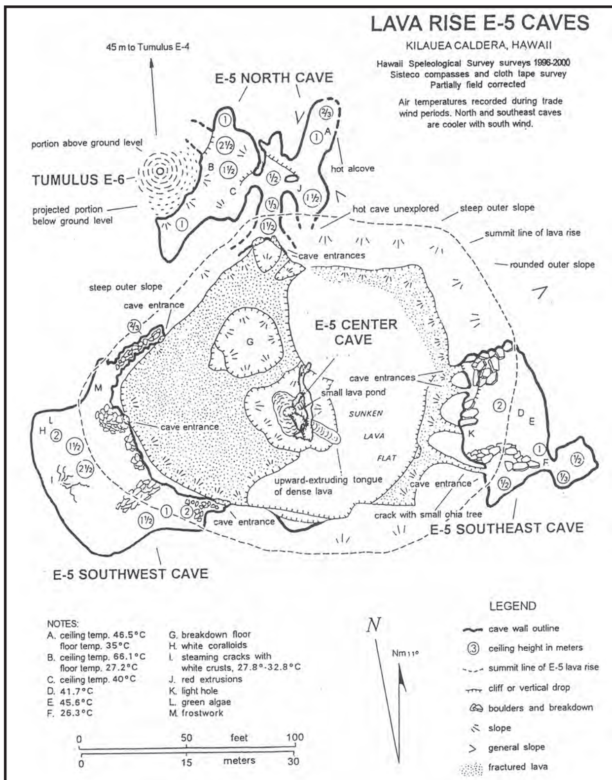
Figure 8: Plan of Lava Rise E-5 Cave.
