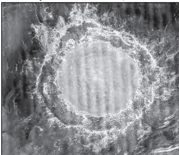
Figure 10: A very detailed image of Lada Regio with many channels, particularly in the middle centre flat area, which could be interpreted as lava tubes. Image from NASA (Courtesy of Windows to the Universe, http://www.windows.ucar.edu ).
