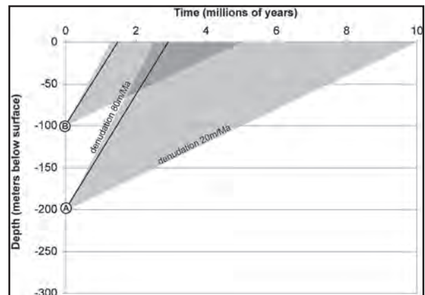
Figure 3: Theoretical persistence of caves in an erosional environment. The length of time that a given cave will exist depends upon the initial depth of formation (position on y-axis) and the denudation rate (slope of line). Gray regions envelope a range of reasonable denudation pathways for two examples. In case A, a cave formed at 200 m depth, the expected lifetime is 2.5 to 10 Ma. For a cave formed at 100 m depth (case B), the lifetime is reduced to 1.25 to 5 Ma. Solid sloping lines are the average denudation rate, 69 m/Ma, for 33 major drainage basins (calculated from data in Summerfield and Hulton, 1994).
