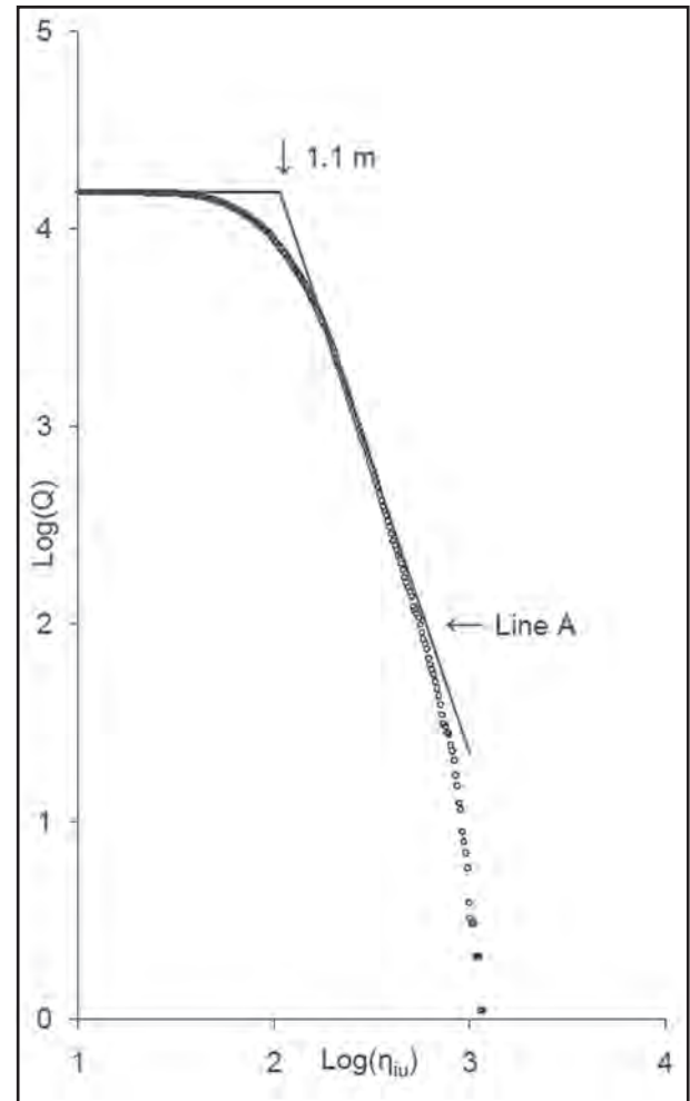
Figure 4: Number of LMEs, Q(\eta) , larger than \eta (cm). The slope in the apparently linear range of a log-log plot approximates D , but is too high due to the truncation of Q(\eta) at large \eta . A correction for truncation is shown by line A, which has slope
