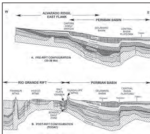
Figure 4: Cross section A shows the Guadalupe Mountains region prior to development of the Rio Grande Rift. Cross section B shows today's structural configuration. Modified from Matchus and Jones, (1984), and Lindsay, (1998, fig. 3).
