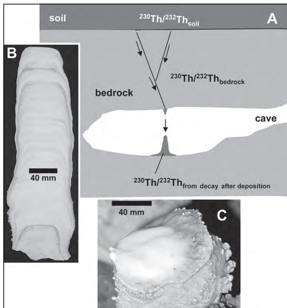
Figure 2: (A) Depositional setting showing two different sources for initial ^{230}\text{Th}/^{232}\text{Th} , a low-value source (soil), and a high-value source (bedrock). (B) Stalagmite BC2. (C) New calcite growth on Stalagmite BC7.
