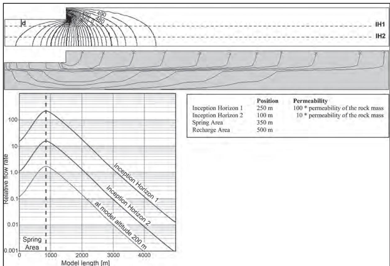
Figure 2: Selected model scenario with one horizontal inception horizon at 250 m (permeability = 100 times that of the surrounding rock mass), and a second inception horizon at 100 m (permeability = 10 times that of the surrounding rock mass). Spring area at model altitude is 350 m and recharge area is at 500 m. The plots illustrate the distribution of hydraulic head (top), flow tracks (middle) and flow rate along the inception horizons as well as at the rock mass at 200 m (bottom) at steady state. The model scenarios show that the vertical flow distribution is proportional to the permeability distribution and is independent of the order of the inception horizons.
