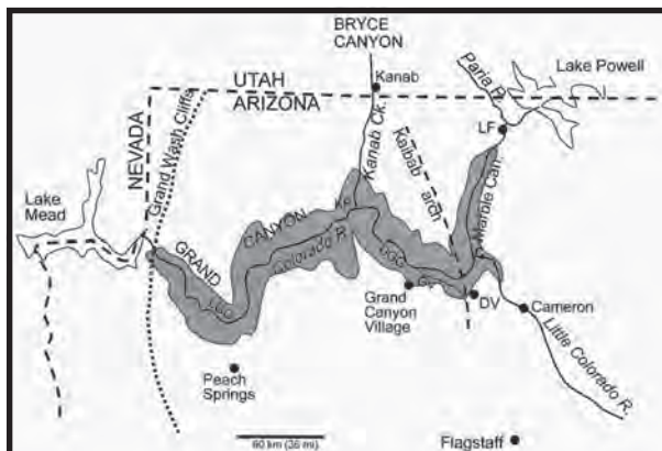
Figure 1: Grand Canyon of northern Arizona, USA. LF = Lees Ferry, C = Confluence, DV = Desert View, GV = Grandview monocline, UGG = Upper Granite Gorge, KP = Kanab Point, LGG = Lower Granite Gorge.
