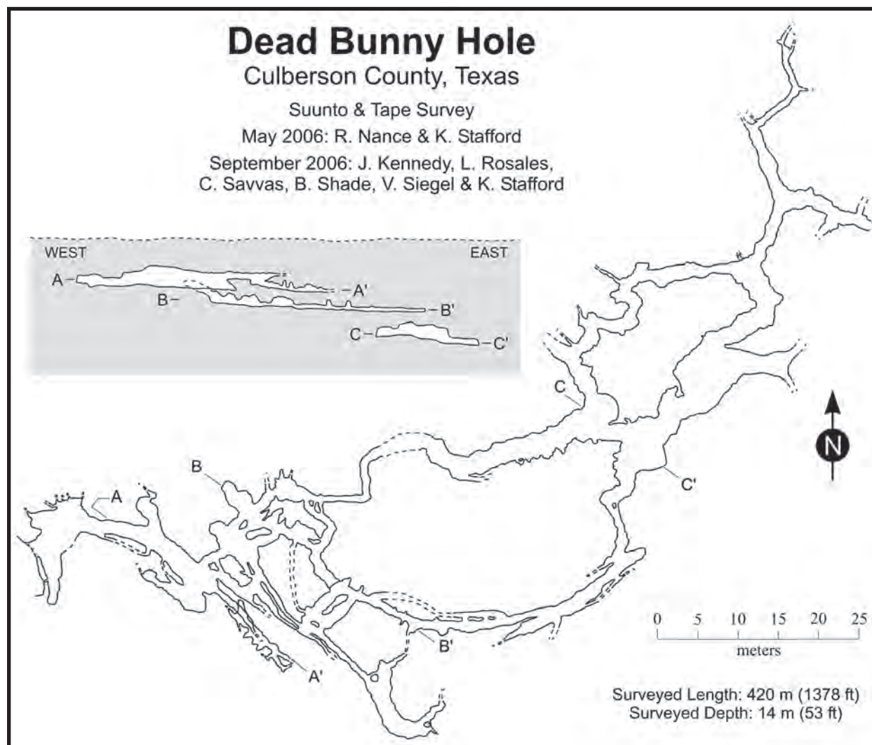
Figure 3. Dead Bunny Hole. Cave was formed by deep phreatic flow in the basal Castile Formation. Epigenic overprinting is currently an active process due to surface breaching in the vicinity of NW-SE trending anticlines.
