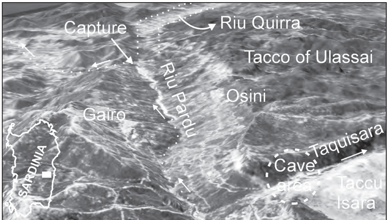
Figure 1: 3D view of Riu Pardu valley looking SSE (from Google Earth). The Taquisara valley cave area (bottom right), the capture of Rio Pardu (top left) and the abandoned Riu Quirra (top middle) are indicated.
