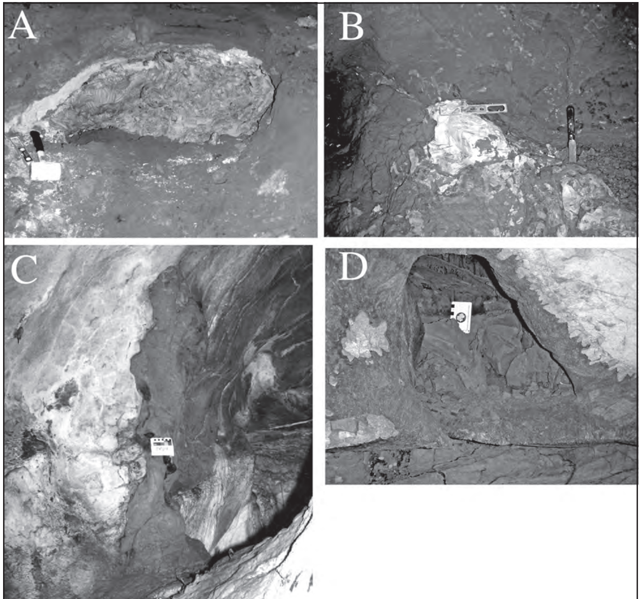
Figure 3: Clay Locations
