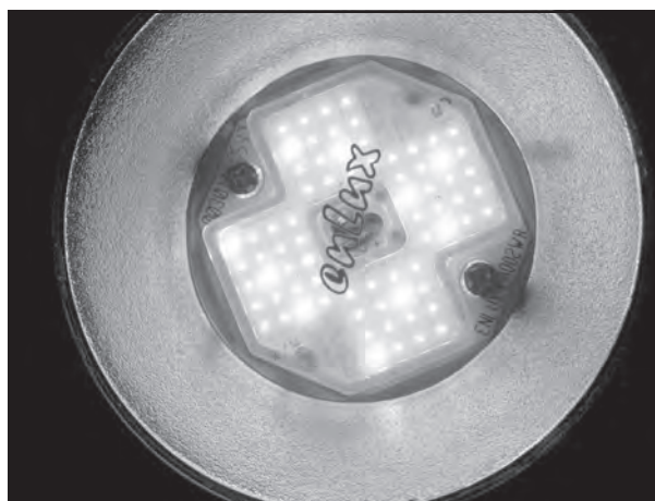
Figure 5: Face of EnLux W2050 bulb showing light engine. The W2050 face has 61 amber, 10 green, and 1 blue LEDs to generate a warm-white light with a color temperature of 2050°K. The brighter LEDs in the picture represent the 10 green LEDs. The width of the light engine is approximately 3 cm.
