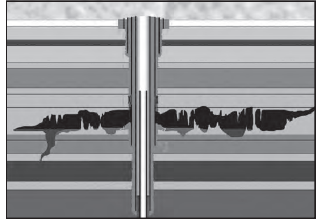
Figure 1-14: Set production liner.
