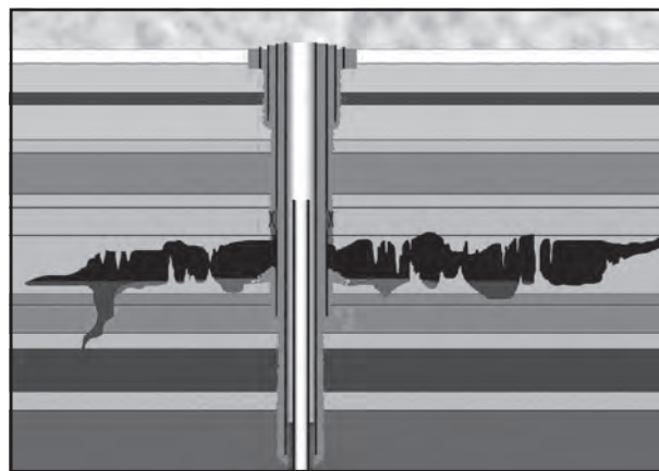
Figure 1-15: Cement liner.
