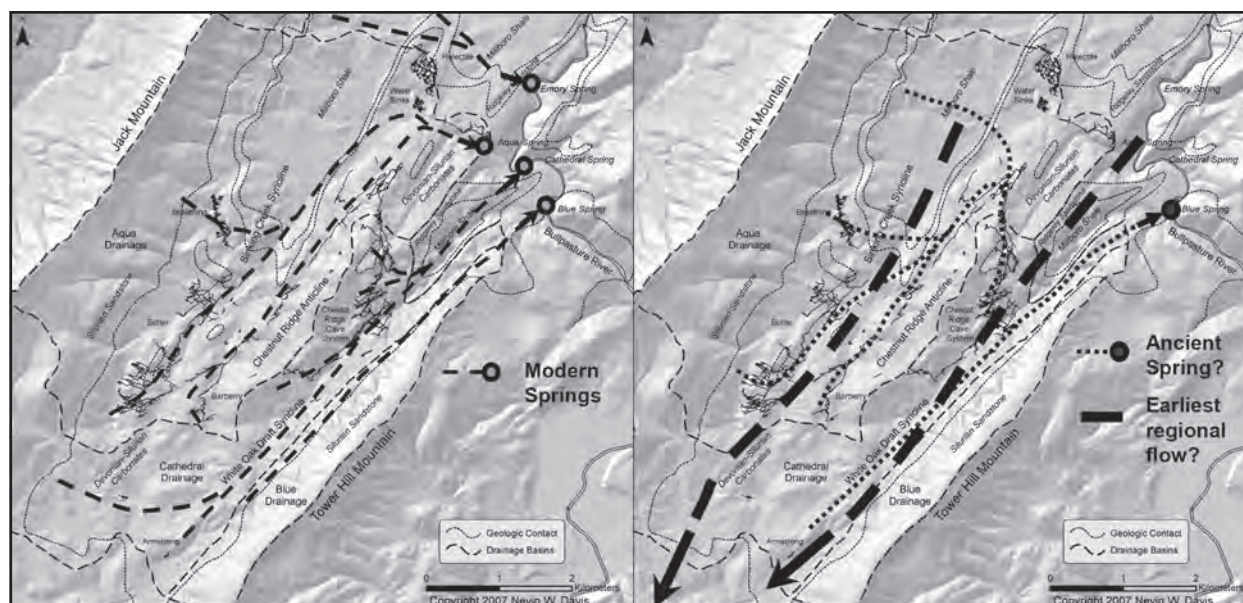
Figure 3: Shaded relief detail map of the Burnsville Cove showing major caves, modern drainage basins, geologic contacts, modern springs and flowpaths (left), and hypothesized ancient spring and earliest regional flowpath (right).
