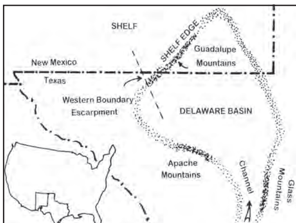
Figure 1: Paleogeography of the mid-Permian in southeastern New Mexico and west Texas. Inset shows the Texas New Mexico area covered by figure.
