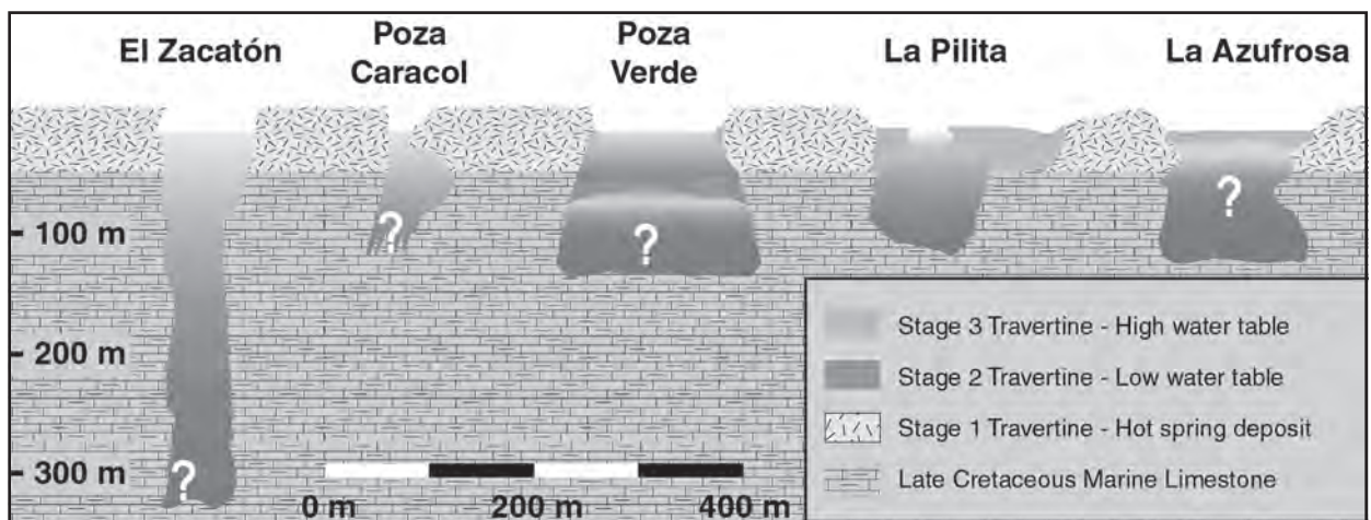
Figure 5: Deep phreatic shafts. Zacaton shaft is one of the numerous windows in the karst aquifer of Tamolipas area (Mexico), reaching a depth of 329 m. Investigation showed nearby volcanoes were the source of \text{H}_2\text{S} . Microbial activity based on sulfur oxidation is present (Gary & Sharp 2006).
