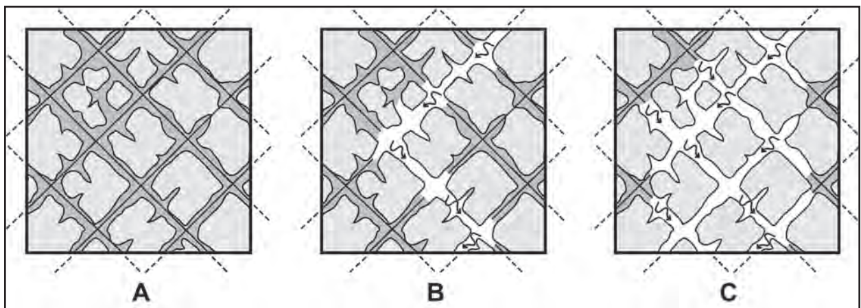
Figure 6: Schematic diagram of evolution from a pseudo-endokarst to a "classic" karst. A - Pseudo-endokarsts are interconnected along the tectonic network exploited by the weathering. There is not enough energy to evacuate the alterite; B - Uplift or valley entrenchment increases the hydraulic gradient. The underground drainage exploits the ghosts and removes the alterite by headward erosion; C - The catchment area of the spring spreads quickly and allows a network of galleries to appear.
