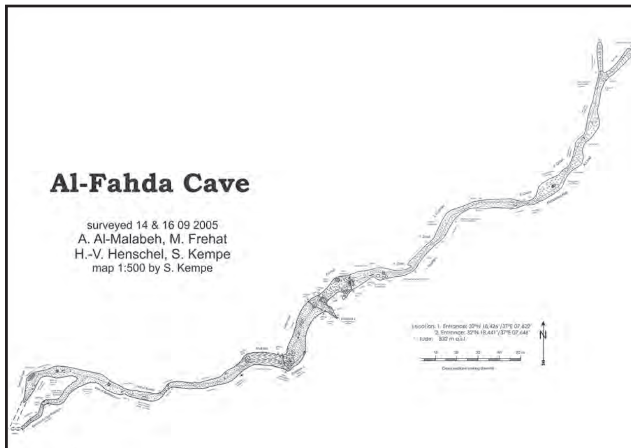
Figure 2: Map of Al-Fahda Lava Cave, longest lava cave in Jordan.
