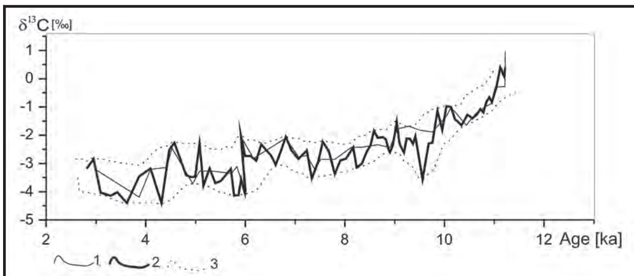
Figure 3: Results of similarity test between high and low density carbon isotopic records from stalagmite JMr 14. 1: Low density (37-points) curve, 2: high density (92 points) curve, 3: 2\sigma confidence bands for a 37-point reconstruction of the 92-point record.
