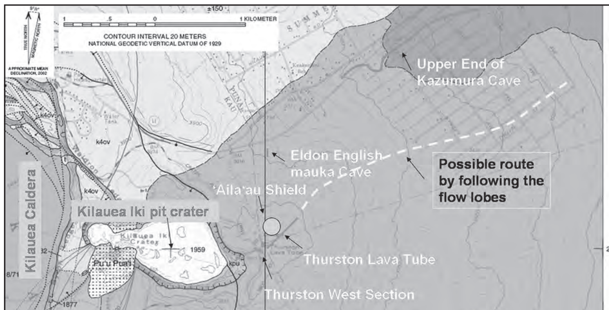
Figure 3: Modified clip of USGS Kilauea geological map (NEAL and LOCKWOOD, 2004).
