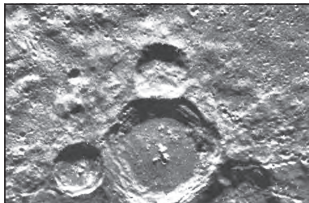
Figure 3: Particular of a group of craters (Mickey Mouse). In the lower left corner, channels can seem to be a series of elliptical hollows as it happens when a lava tube collapses.
