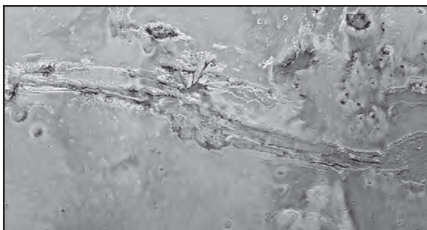
Figure 11: Another view of the Vallis Marineris; various structures, probably lava tubes, run parallel to the valley. Image from NASA (courtesy of Windows to the Universe, http://www.windows.ucar.edu ).
