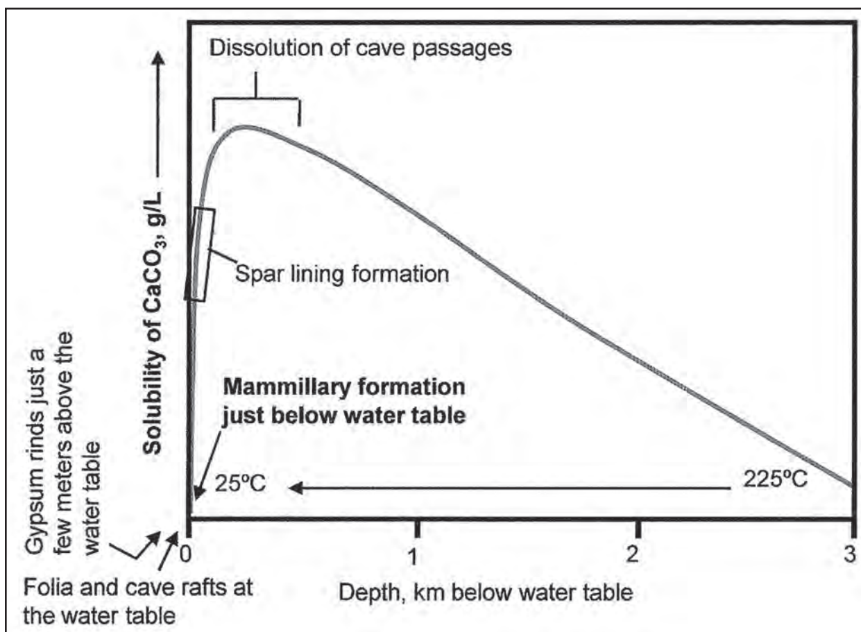
Figure 2: As convective water rises and cools, the solubility of calcite gradually increases so that small caves dissolve in the phreatic “solutional zone.” As the water table descends, caves formed in the solutional zone are shifted into the “depositional zone.” When this happens the solubility of calcite drops sharply due to the loss of \text{CO}_2 and solutions change from aggressive to precipitative. Since the loss of \text{CO}_2 is very slow in the deeper phreatic zone, large spar crystals line previously formed cave passages. Just below or near the water table in the shallow phreatic zone the loss of \text{CO}_2 is much more rapid and therefore fine-grained mammillary coatings form instead of spar linings. At the water table-air interface folia and cave rafts form, and just above the water table replacement gypsum rinds form. After Dublyansky (2000).
