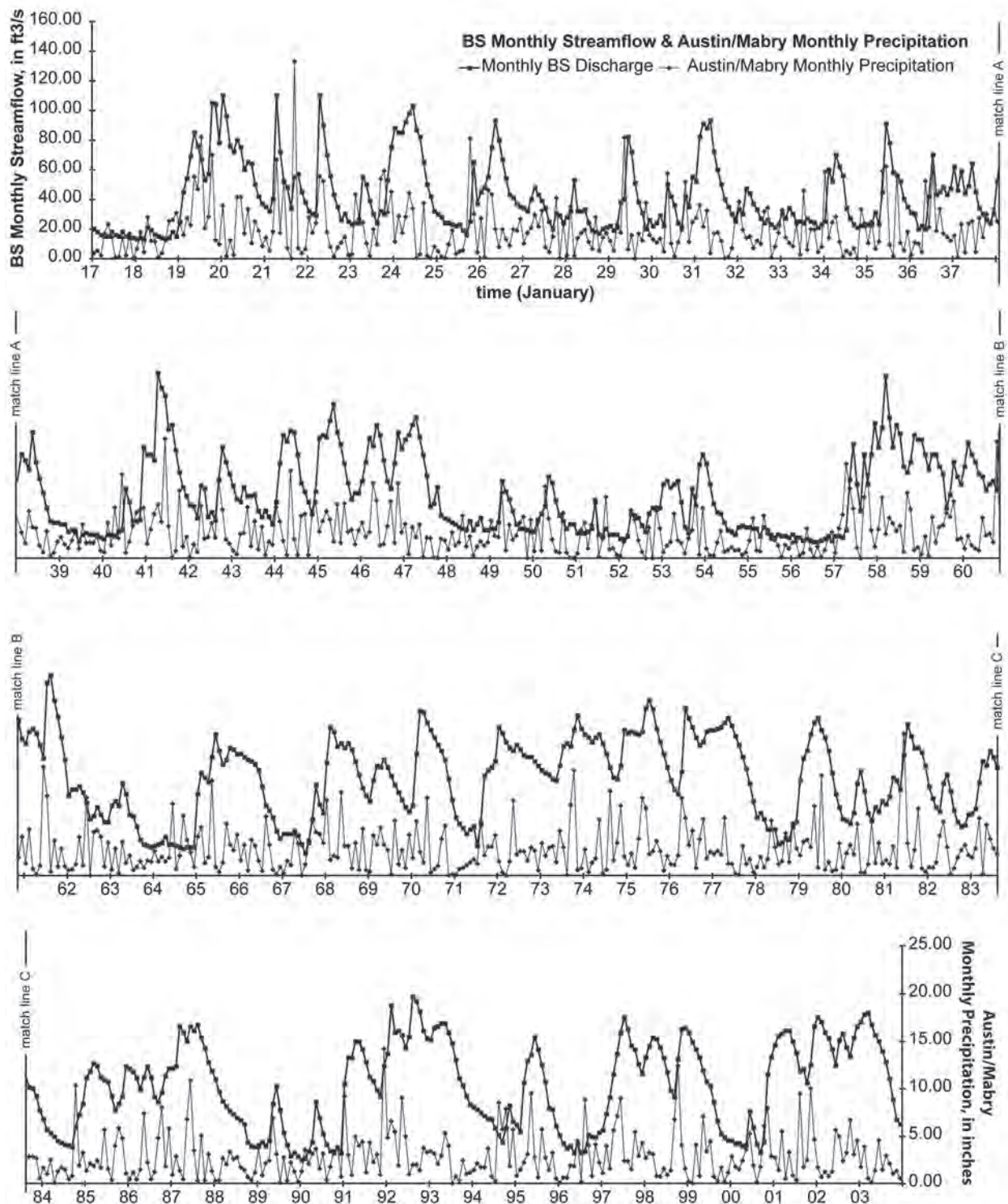
Figure 2: Monthly Barton Springs flow and precipitation data.
