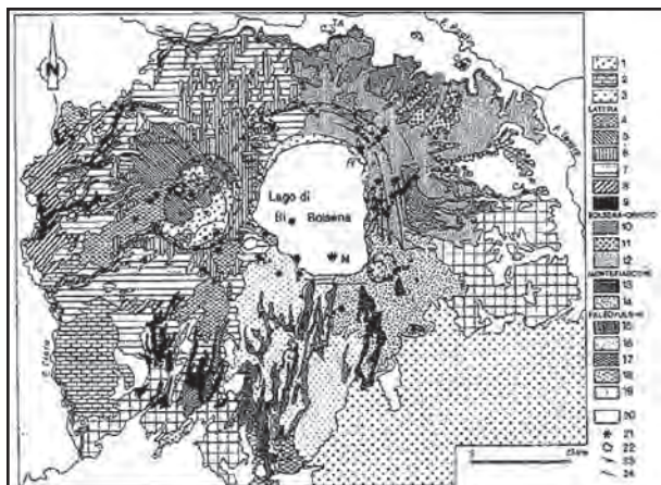
Figure 1: Geological map of the Volsinean system. The tunnel is located in the circled area.
