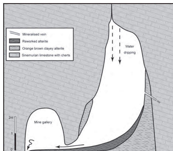
Figure 5: Schematic section of a vertical pocket. Ghost rock has partially eroded since the opening of the mine.
