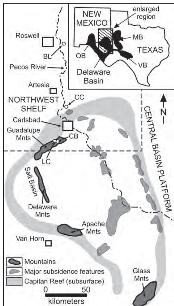
Figure 1: Map of Delaware Basin showing the geographic relationships between the Capitan Reef, major subsidence features and the Pecos River. BL = Bottomless Lakes State Park, CC = Coffee Cave, CB = Carlsbad Cavern, LC = Lechuguilla Cave, OB = Orogrande Basin, MB = Midland Basin, VB = Valverde Basin (adapted from Klimchouk, 2007).
