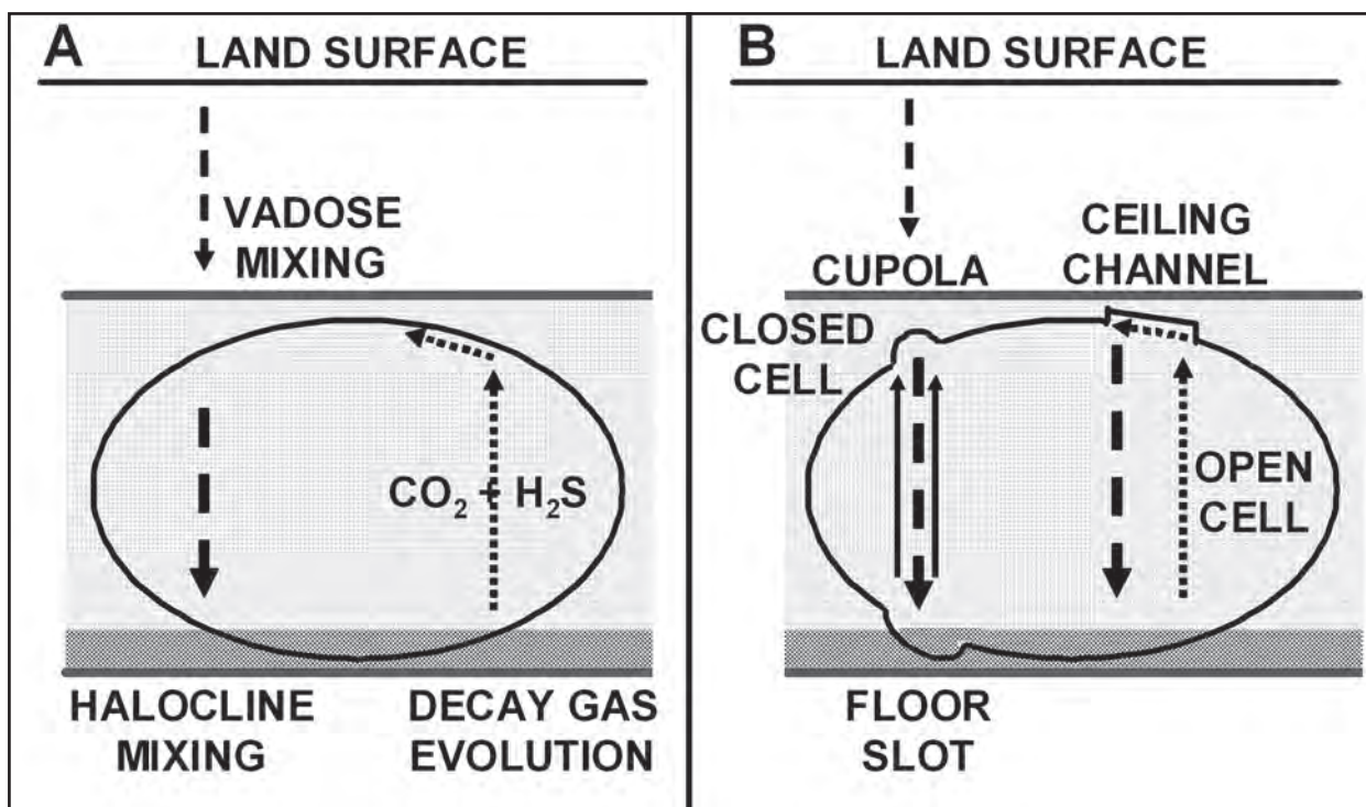
Figure 3: Diagrammatic representation of possible dissolutional processes within flank margin caves that can produce bedrock morphologies similar to those found in confined hypogenic caves. A) Mixing locations (left), and decay of organics trapped at the halocline to produce \text{CO}_2 and \text{H}_2\text{S} (right). B) Closed cell convection creates cupolas and floor dissolution (left), open cell convection creates ceiling channels and chains of cupolas (right). See text for a full discussion.
