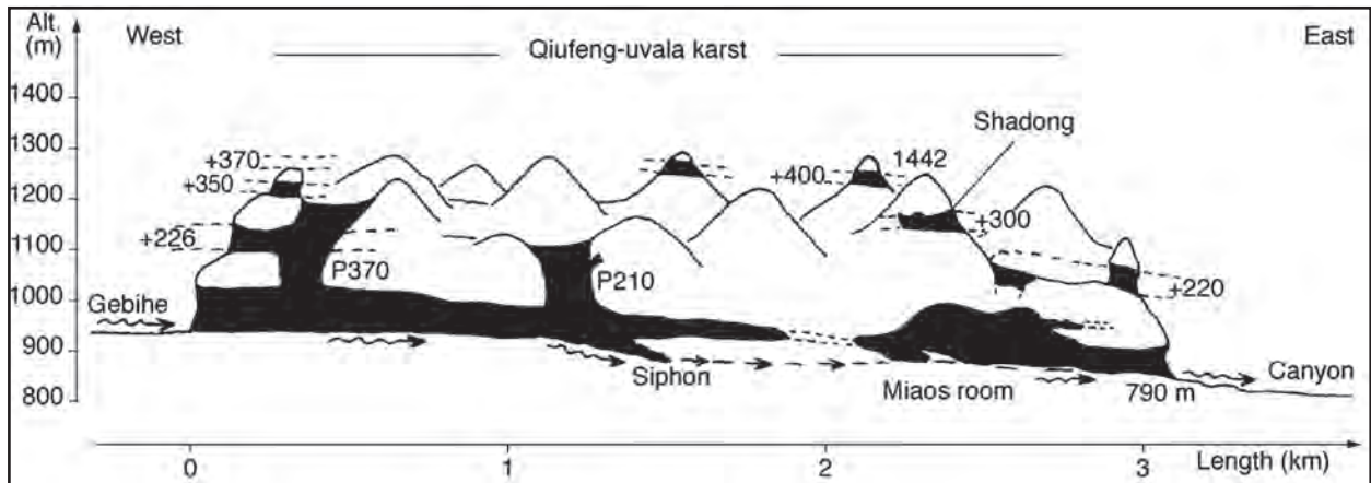
Figure 8: Synthetic section of the Gebihe staged tunnel-cave (Ziyun County, Guizhou).
