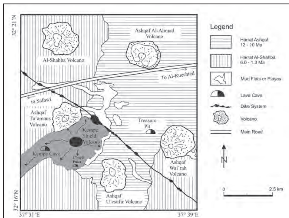
Figure 4: Geological map of the Kempe Volcano (Map by Al-Malabeh and Kempe based on Field observations and Google Earth images).
