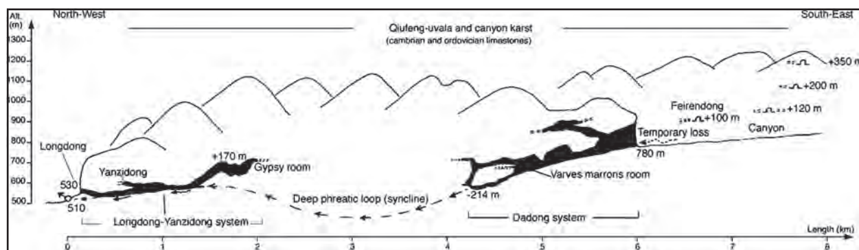
Figure 6: Synthetic section of the Dadong-Longdong tunnel-cave (Wufeng County, Hubei). We notice a saturated level in the syncline part.
