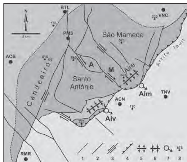
Figure 2: Sketch of Estremenho limestone massif. 1 - Topographic limit; 2 - Fault; 3 - Strike-slip fault; 4 - Arrife thrust fault; 5 - Aire anticline; 6 - Monsanto syncline; 7 - Karst spring; 8 - Altitude asl (m); Dashed square A: Alvados polje (represented in Fig. 4); Dashed square M: Minde polje (represented in Fig. 3); Dark grey texture: Jurassic limestone of Estremenho massif; Medium grey texture: mainly Mesozoic detrital rocks; Light grey texture: Tagus basin Cenozoic formations. ACB - Alcobaça; ACN - Alcanena; BTL - Batalha; PMS - Porto de Mós; RMR - Rio Maior; TNV - Torres Novas; VNO - Ourém. Alm - Almonda spring; Alv - Alviela spring.
