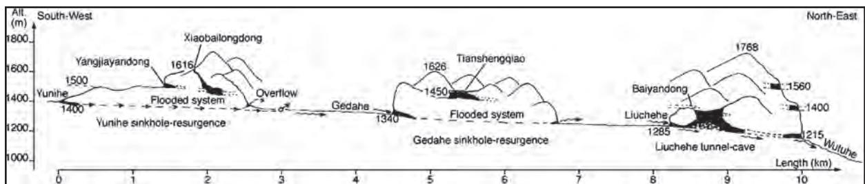
Figure 9: Synthetic section of the tunnel-caves system of Wutuhe (Panxian, Guizhou).
