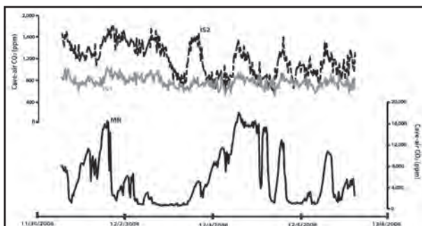
Figure 2: A representative sample wintertime CO 2 fluctuations in Inner Space Cavern and Maple Run Cave. Distance of loggers from the cave entrance and r 2 values for correlations between CO 2 and surface temperature and pressure are given in Table 1.
