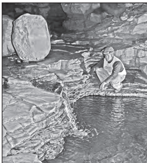
Figure 3: In areas of active stream flow, smoothing of the rock demonstrates the humic-acid dissolution process.
