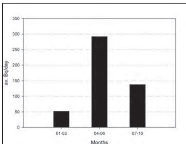
Figure 3: Average Rn concentration in Bq/day.
