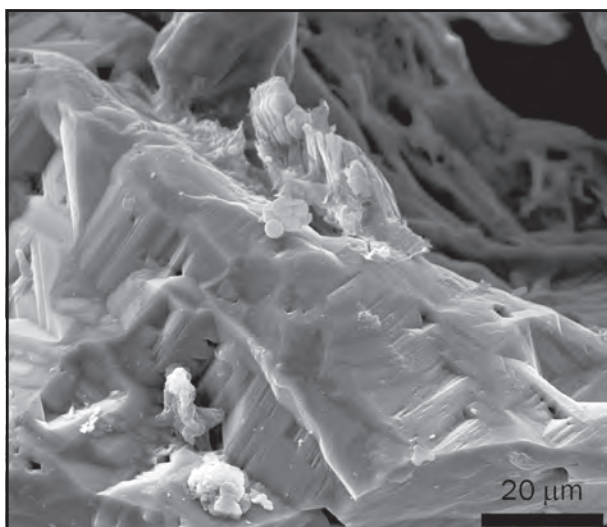
Figure 2: An SEM image of quartz sand grains taken from Roraima Sur Cave. The triangular-shaped pits are indicative of chemical weathering. A cluster of what appear to be bacterial cells is present in the upper-middle.
