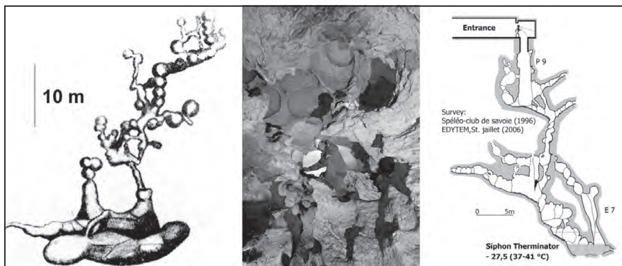
Figure 6: Upwardly dendritic caves. Left: Sátorkő-pusztá Cave, Hungary, has been used to represent thermal speleogenesis. Upwardly dendritic spheres develop above a basal chamber (survey in Ford & Williams 1989). Center: stacked up spheres in Serpents Cave, France, which is close to Chevalley. Right: Chevalley shaft, France (Audra et al. 2007).
