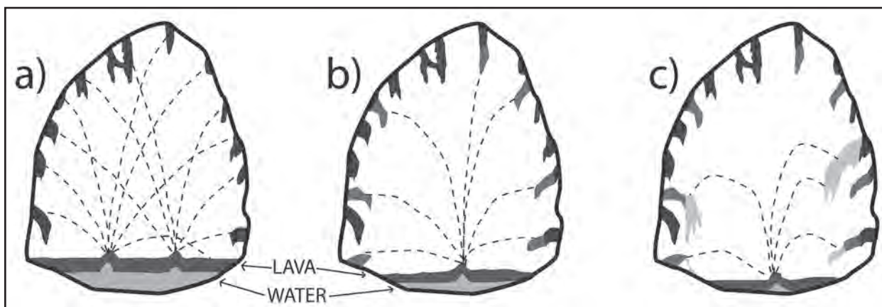
Figure 2: A series of diagrams, not to scale, illustrating the cross section of a lava tube, showing what could happen when lava fountains in a confined space: a) shows a pool of water trapped underneath flowing lava, turning to steam, and forcing random fragments of lava to hit the walls and ceilings in random trajectories; b) shows more fragments hitting walls and other fragments of lava, resulting in stalactite-like speleothems; c) The fountain is losing steam and trajectories are not as high. Stalactites grow towards the source of the fountain, and some are long enough to shadow the areas behind them.
