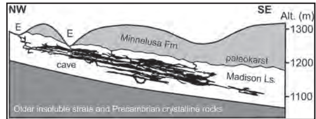
Figure 3: Geologic profile through Wind Cave. E = entrance.
