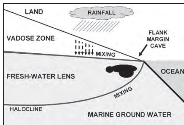
Figure 2: Diagram of the fresh-water lens in a carbonate island, showing the upper and lower lens boundaries and mixing areas, and the development of flank margin caves under the flank of the enclosing landmass, in the distal margin of the lens. The vertical scale has been exaggerated, the lens does not dip as steeply as shown.
