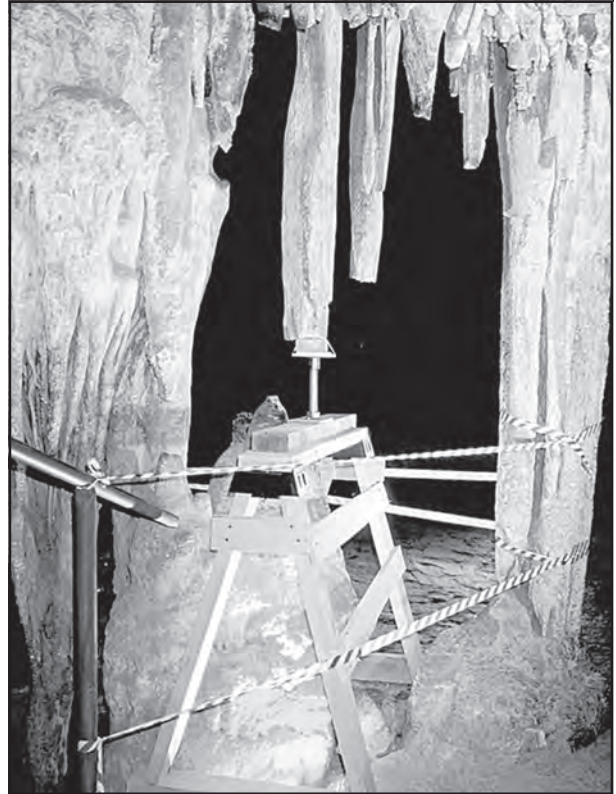
Figure 6a: (Before) and Figure 6b: (Midway through the repair) In the second image, after the reattaching the upper piece to the ceiling, we cordoned off the support jack for visitor safety and left it in place for several weeks to assure proper curing of the archival epoxy. Photo by Val Hildreth-Werker.
