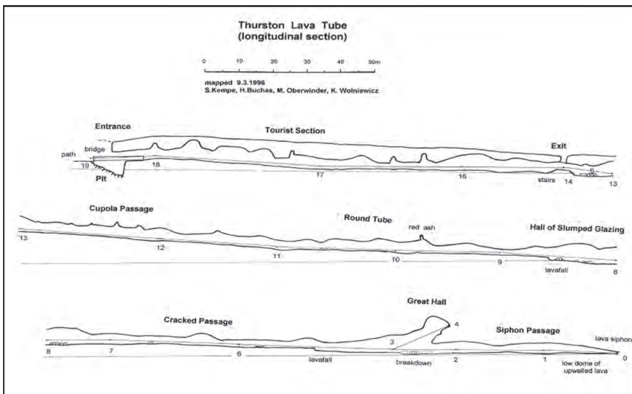
Figure 2: Longitudinal section of Thurston Lava Tube.
