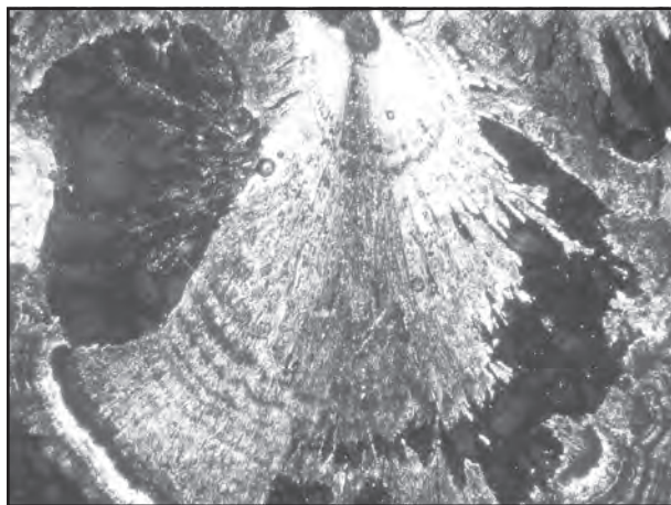
Figure 4: Photo of thin section in polarized light showing an aragonite bud (grey), 1 mm wide, replaced partially by opal (black). Residual aragonite needles are visible in opal because of dissolution. Mechta Cave (Baikal, Russia).
