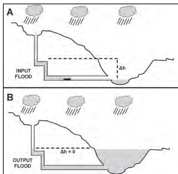
Figure 4: Comparison of input and output flooding. A) Input flooding can fill all or part of the cave, but high flow velocities may also be present because the hydraulic head ( \Delta h ) is large. B) Output flooding creates a zero head condition ( \Delta h = 0 ), and stagnant flow conditions in much of the cave. This setting could allow slow vertical flow mechanisms to produce bedrock dissolutional morphologies similar to those seen in confined hypogenic caves.
