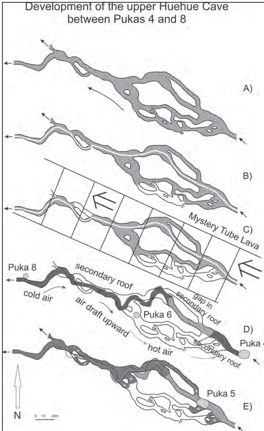
Figure 2: Detail of the ground plan of the Huehue Cave illustrating how a primary maze of parallel lava threads (A) was drained until the master trunk that cut down fastest remained (E). (A) Initial pattern of lava tunnels, flow was from right to left in up to five parallel conduits. (B) The southern-most conduits were drained first. (C) Further downcutting reduced the number of active conduits to three. At the same time, lava from a parallel flow (Mystery Flow) covered the area. (D) Only one tunnel remained (following the thick line in B and C), its bed 2 m below the original surface. The added overburden caused collapse of pukas (labeled 8, 6 and 4) the breakdown of which was removed by the lava river. Now external air began flowing uphill from Puka 8 to 4. As a consequence a secondary ceiling froze out above Puka 8 and below Puka 8. (E) Various spill-events reinforced the secondary roof, even spilling into the already drained upper conduits, closing the northern-most one. These spilled lavas were oxidized by the passing surface air and attained various shades of red caused by the crystallization of very fine-grained hematite. The last event was the collapse of puka 5 while the tube cooled. Its material is still in place.
