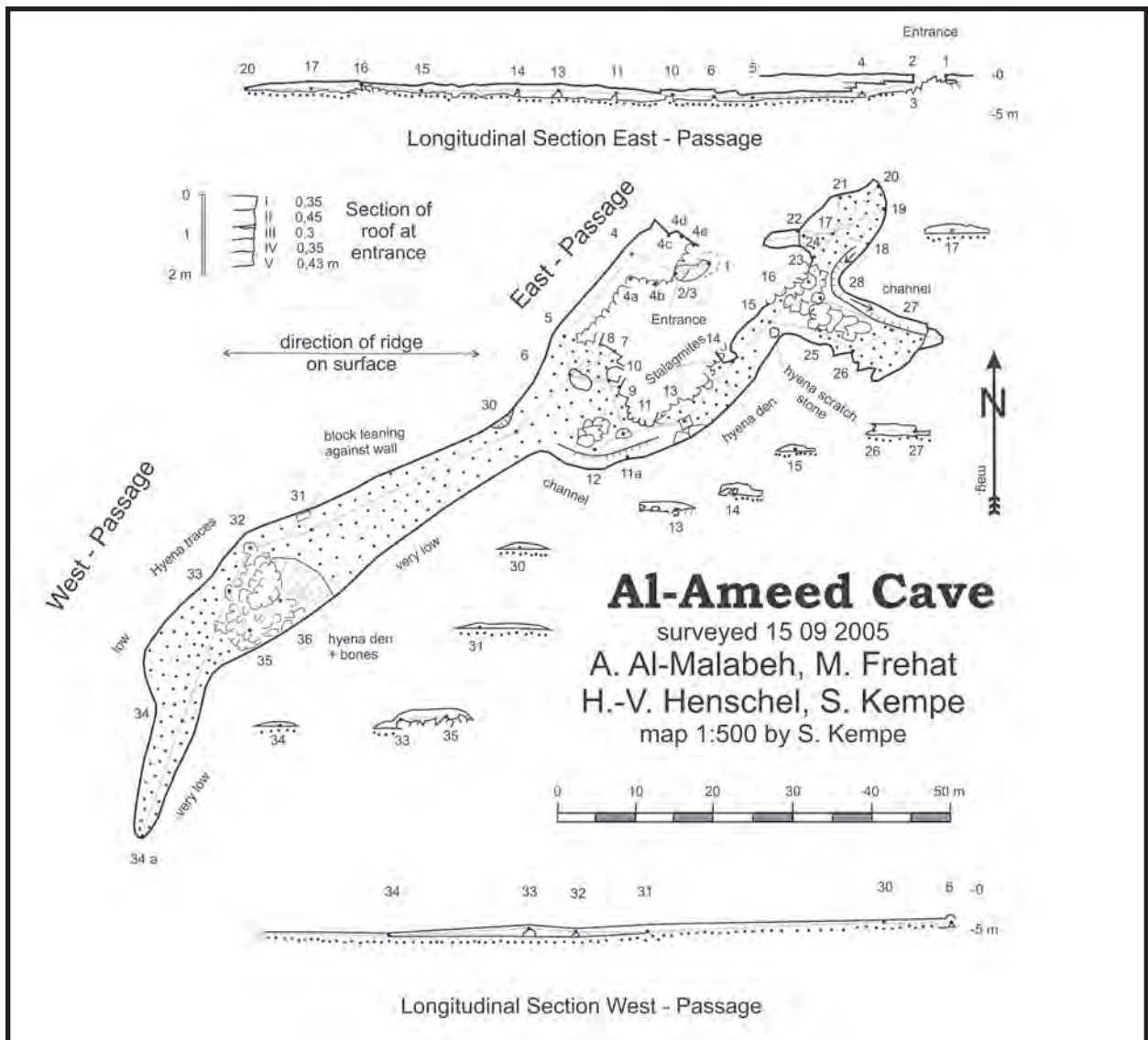
Figure 6: Map of Al-Ameed Cave.
