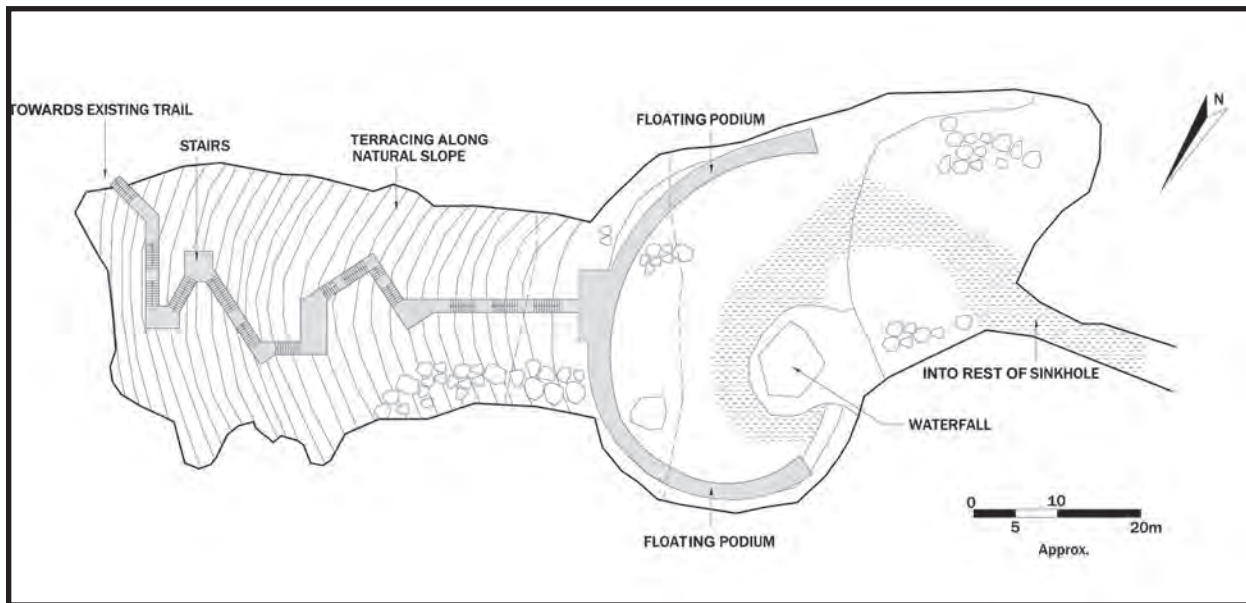
Figure 6: Schematic representation of proposed descent into pothole with stairway path along artificial terraces.
