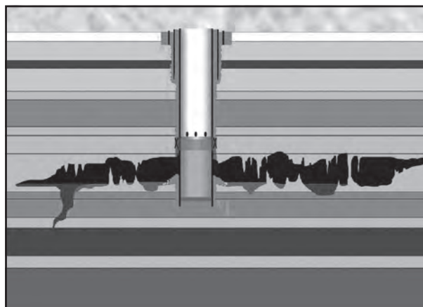
Figure 1-10: Cement second stage to surface above cave.
