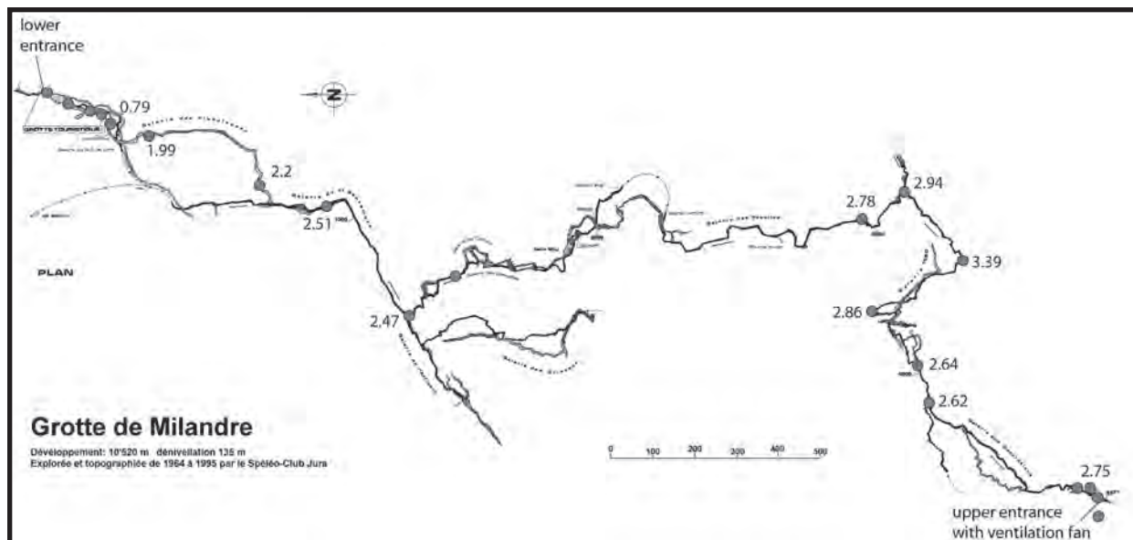
Figure 4: Approximate distribution of CO 2 concentrations in the Milandre Cave before the beginning of the ventilation experiment in September 2008.
