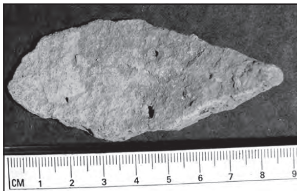
Figure 7: One of many pointed or sharp-edged basalt fragments found near station 5.
