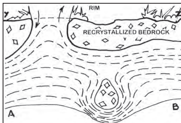
Figure 5: Wall rock retreat due to condensation. If two rock surfaces, A-B and Y-Z are at different temperatures, the amount of heat flow will depend on the temperature gradient ( DT/d ). Small variations in thickness may result in locally higher rates of heat flow, resulting the progressive accentuation of surface topography.
