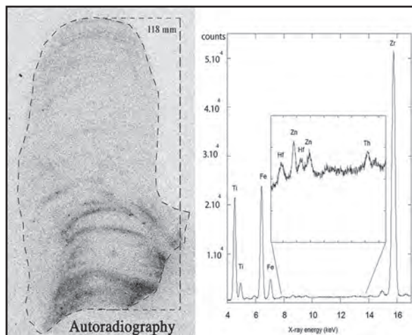
Figure 5: Autoradiography of Trou Noir stalagmite (left) and \mu -XRF spectrum of a zircon (right). The radioactivity is due to thorium.
