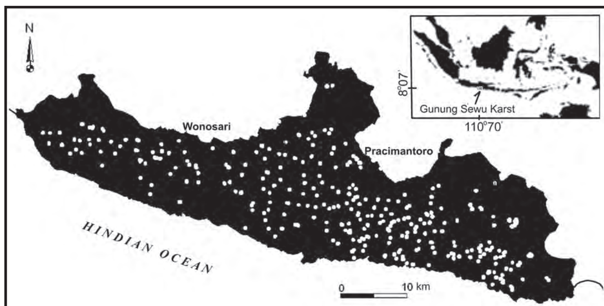
Figure 1: Distribution of telaga in Gunungsewu Karst (compiled from topographical maps).
