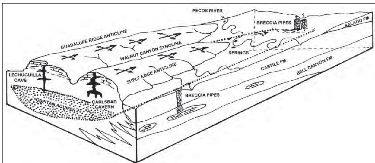
Figure 2: Relationship of regional structure to the aquifer and location of major caves. The erosion of the Basin and Range uplift has progressed more slowly than the development and integration of the Capitan Aquifer, which is everywhere below the level of the mountain front, forcing all flow through the springs and breccia pipes in the Pecos River Valley.
