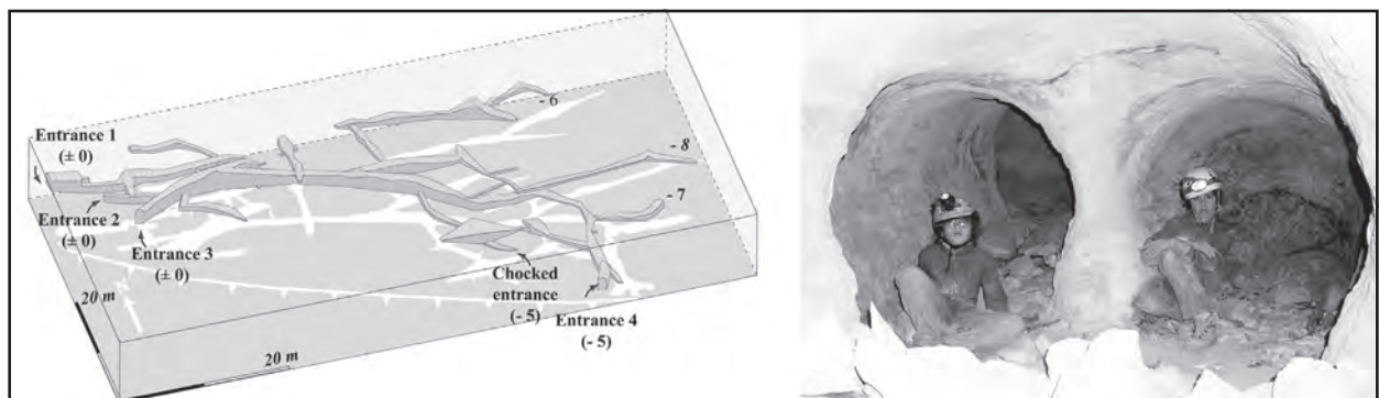
Figure 4: A sub-type of the 3D maze, the 2D maze confined under an inclined impervious roof. Grotte de Saint-Sébastien (France). The dip is towards the SE, water used to well up towards the left.
