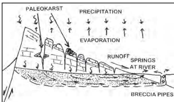
Figure 1b: Hydrology of the Guadalupe Mountains. The Capitan is everywhere lower than the canyon bottoms, forcing water to resurge along the river.
