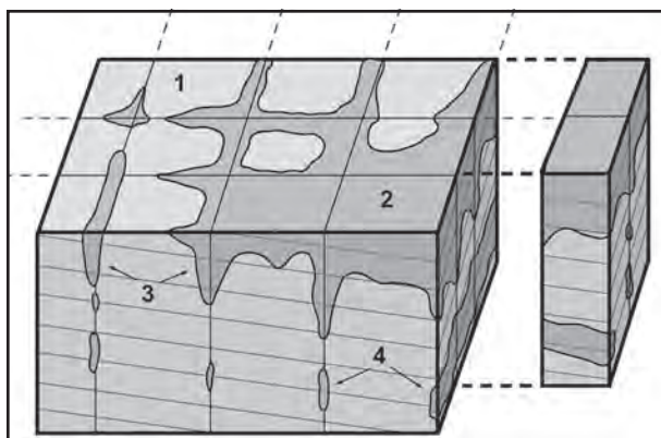
Figure 2: Schematic diagram showing the different types of ghost rocks. 1 – competent rock; 2 – large area of ghost rocks, with overlying voids formed by compaction of the alterite; 3 – pockets and corridors developed along discontinuities and fractures; 4 – ghost rocks under a secure roof: the pseudo-endokarst.
