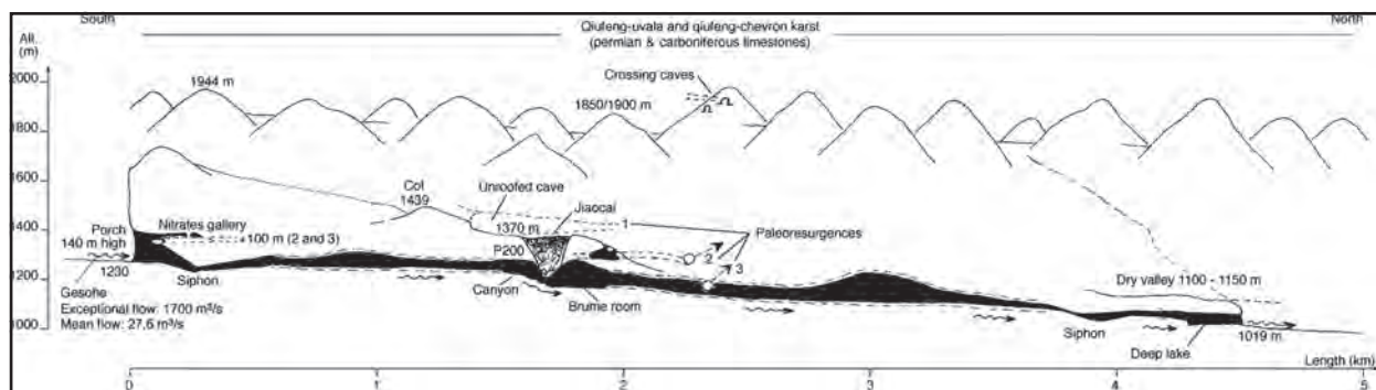
Figure 11: Synthetic section of the Geshe tunnel-cave (Panxian, Guizhou).
