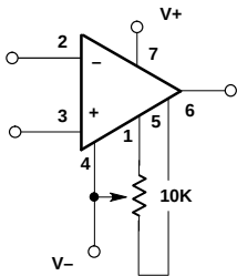
Offset Null Circuit
